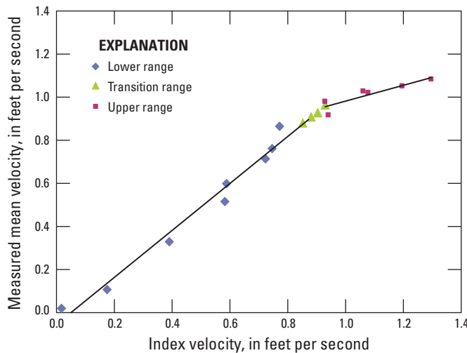
Figure 34. Two linear segments and the points used to define the transition between each segment for the compound-linear rating example.
