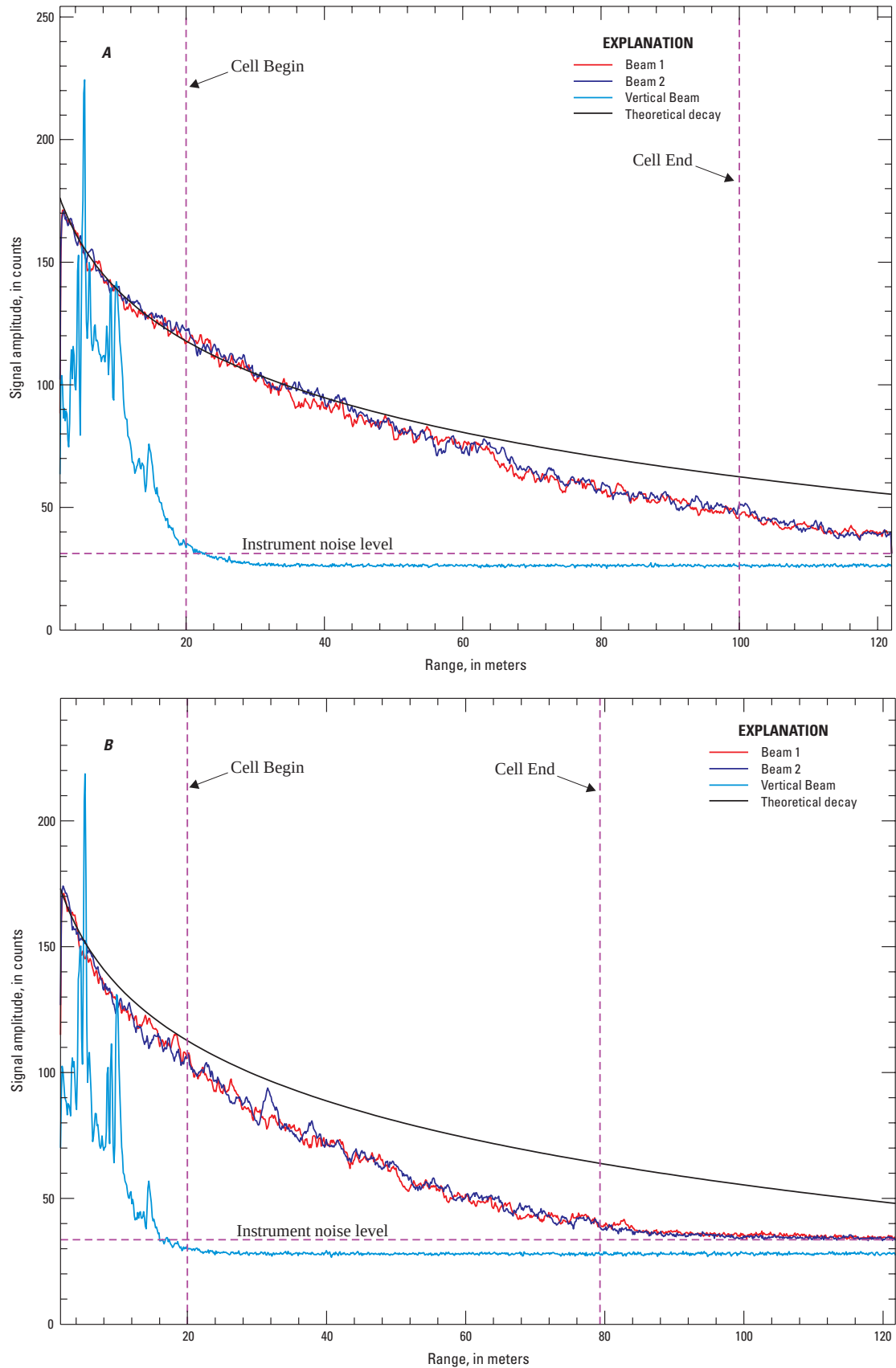
Figure 11. Beam checks for the same site with (A) acceptable signal amplitudes to the end of the measurement volume in October 2009, and (B) decreased signal amplitudes in January 2010.
