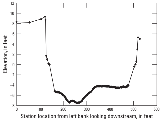
Figure 18. Example of a channel cross-section shape.
