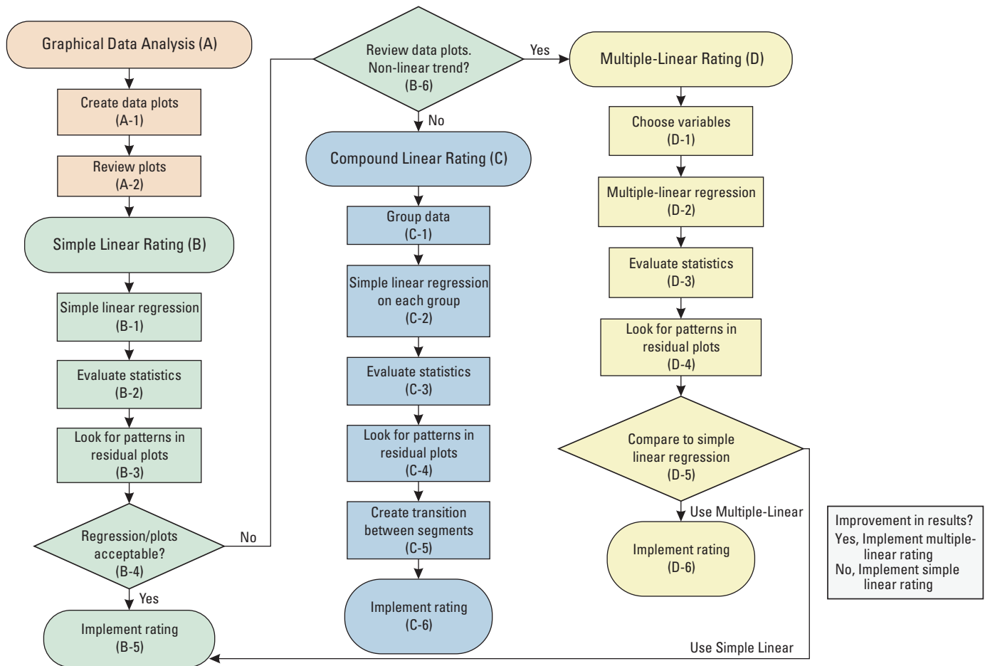
Figure 23. Steps for creating an index rating.
