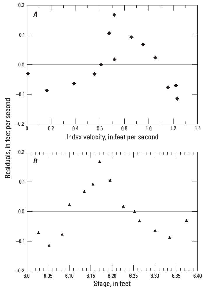
Figure 37. Patterns in plots of residuals from simple-linear regression with (A) downstream index velocity and (B) stage.
