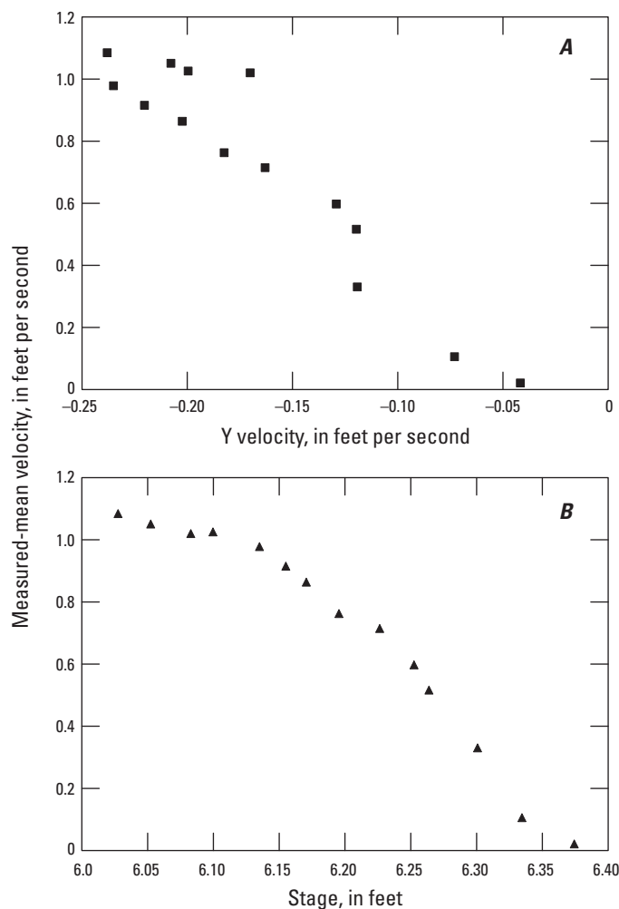
Figure 36. Patterns in plots of (A) Y velocity and (B) stage with measured-mean channel velocity.
