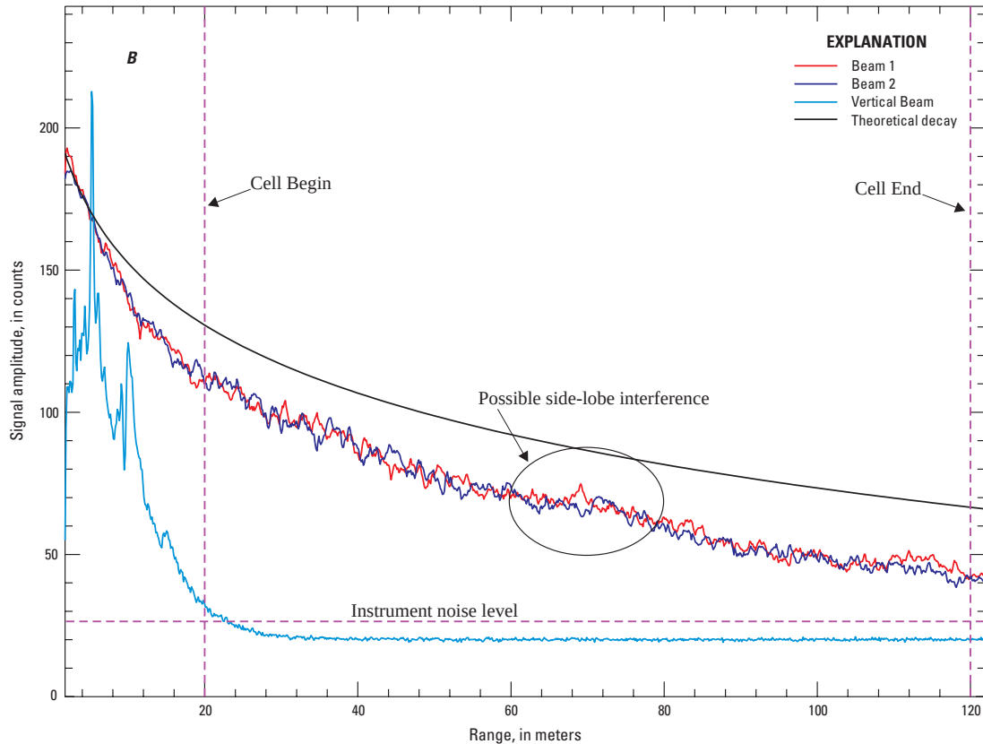
Figure 16. Results of beam checks showing data collected with (A) objects in the measurement volume, (B) side-lobe interference, (C) failed transducers, and (D) a school of minnows in the measurement volume.
