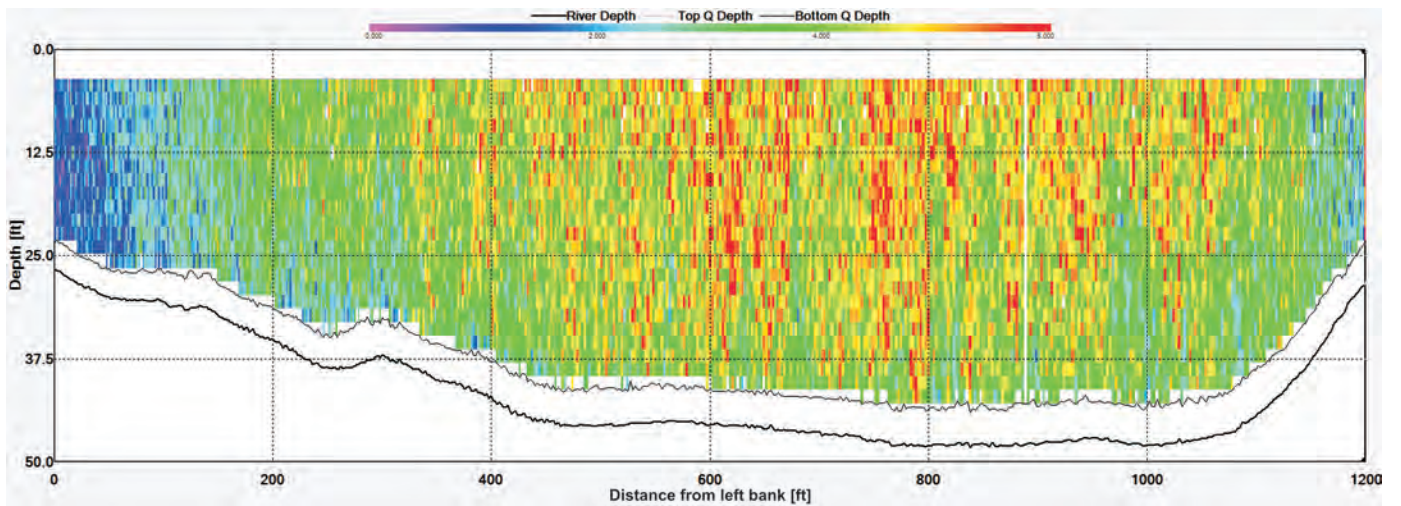
Figure 2. Channel cross section looking downstream with a uniform channel shape and a uniform velocity distribution from an ADCP reconnaissance measurement.
