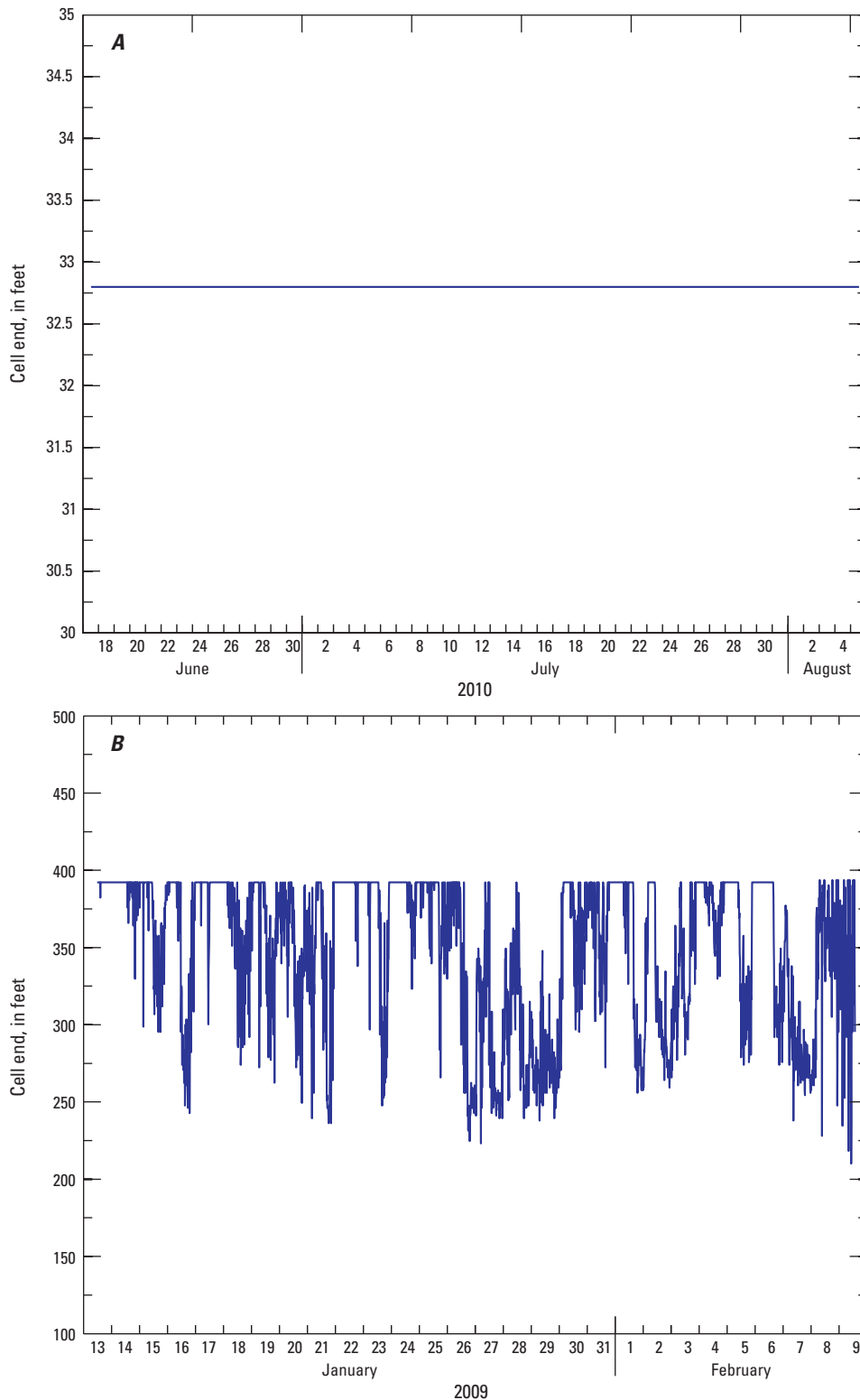
Figure 4-7. Sidelooker ADVm range-averaged measurement volume time-series data with (A) no change in cell end and (B) substantial changes in cell end.
