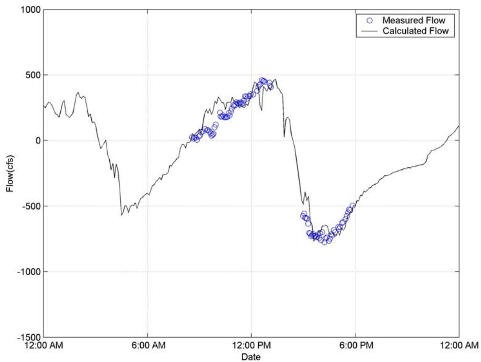
Figure 3-3. Measured and Calculated Flow on May 18, 2015
