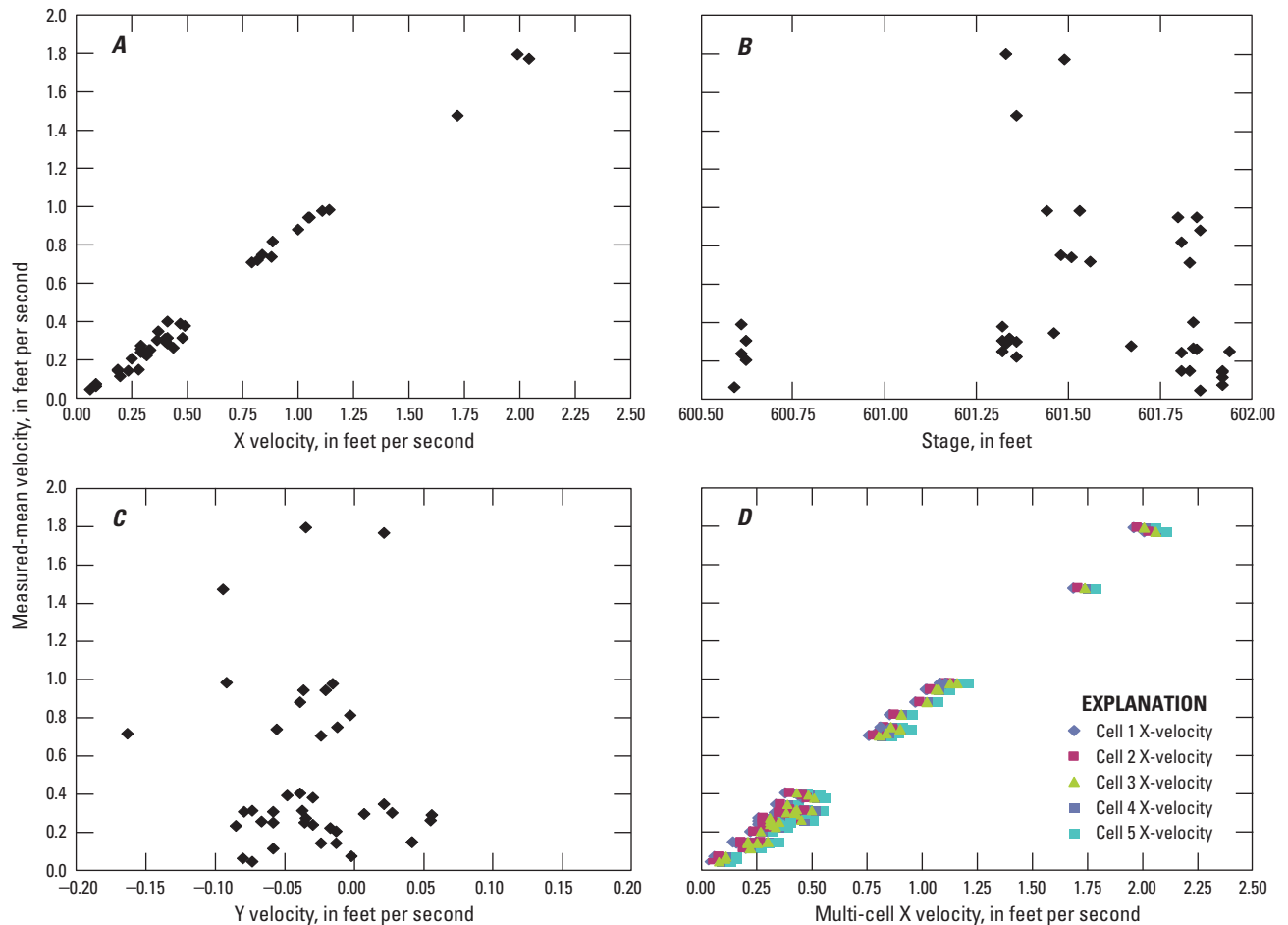
Figure 28. Plots of (A) range-averaged X velocity, (B) stage, (C) Y velocity, and (D) multi-cell X velocity with measured-mean velocity for simple-linear rating example.
