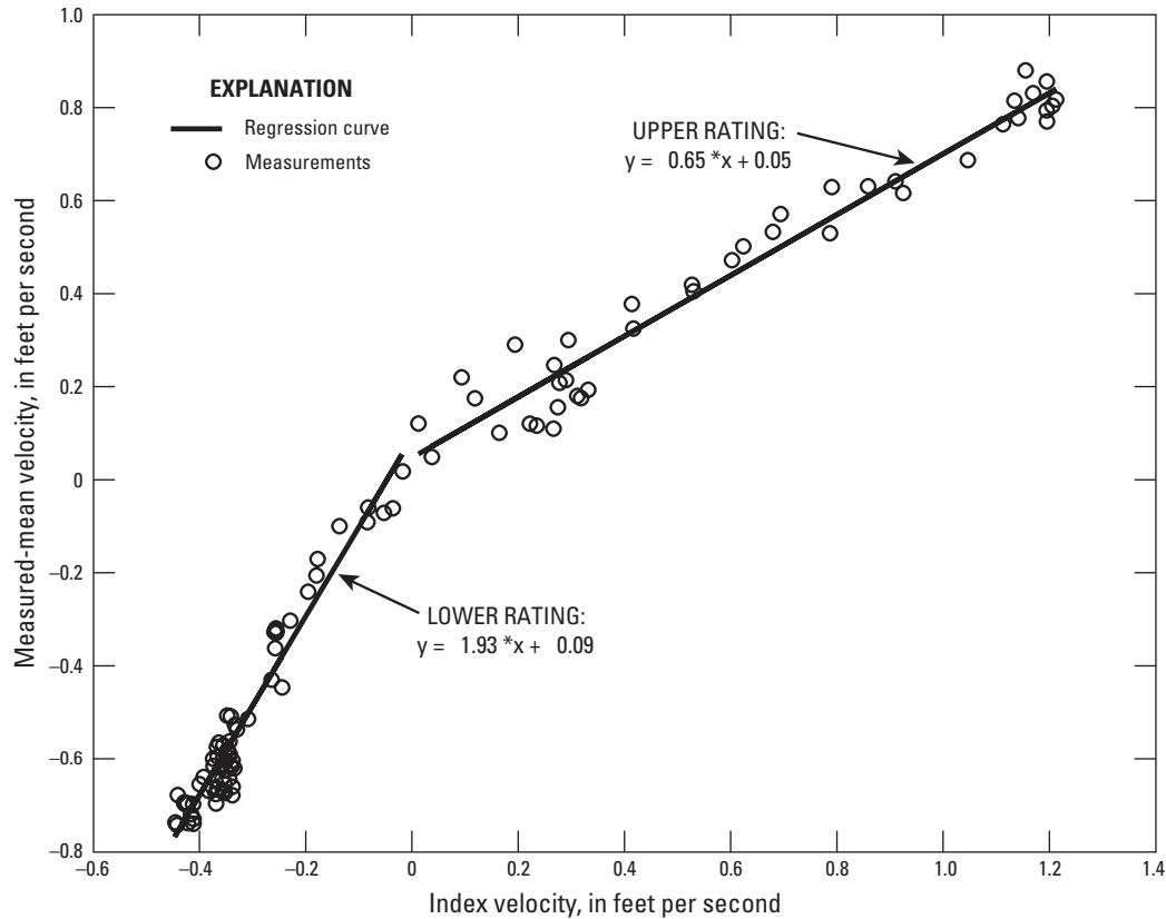
Figure 30. Example of a compound-linear index rating (from Ruhl and Simpson, 2005, p. 23).
