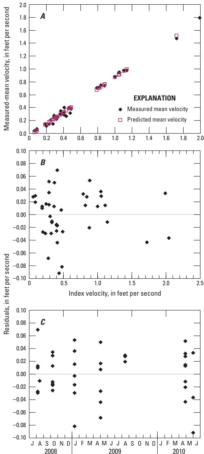
Figure 29. Plots of (A) measured-mean velocity and predicted mean velocity and (B) regression residuals with index velocity, (C) and regression residuals with measurement date.
