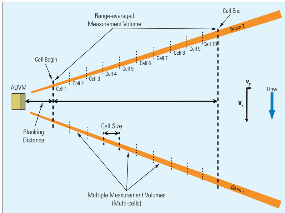
Figure 8. Generalized measurement volumes for a sidelooker ADVM.
