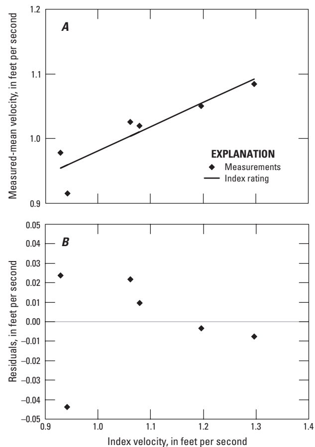
Figure 33. Plots of (A) measured-mean velocity and index velocity, and (B) regression residuals with index velocity for upper range of compound-linear rating example.
