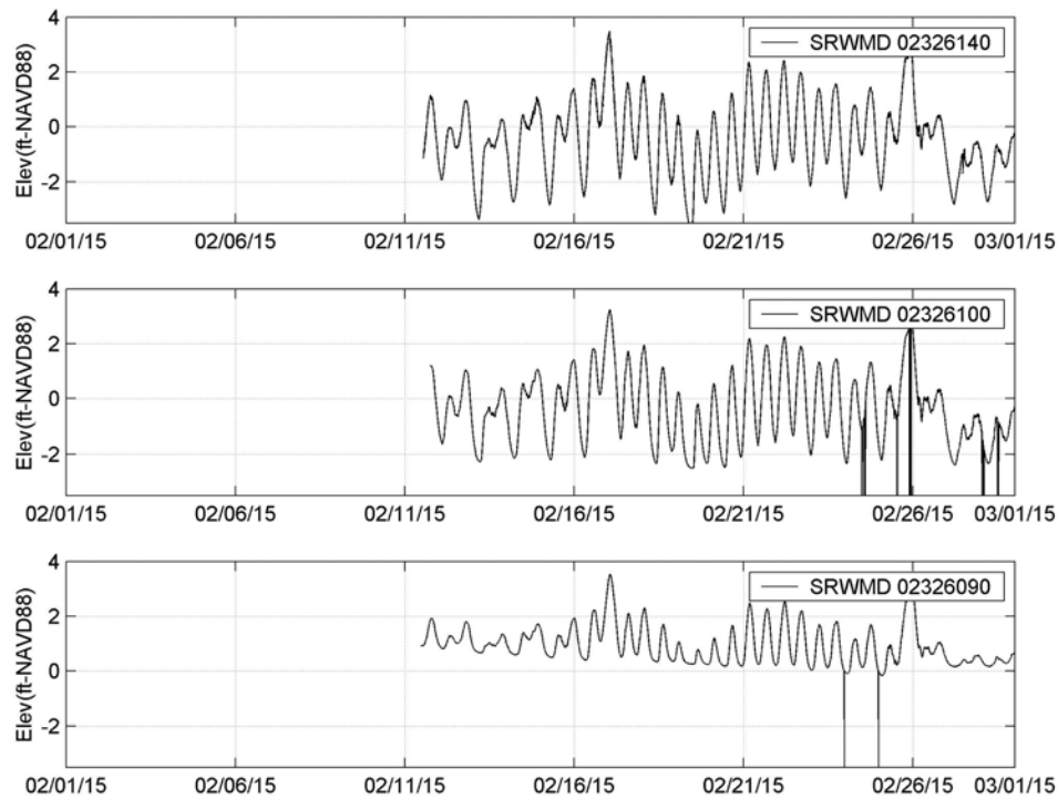
Figure 4-1a. Measured Water Level at Station 02326140, 02326100, 02326090 (February 2015)
