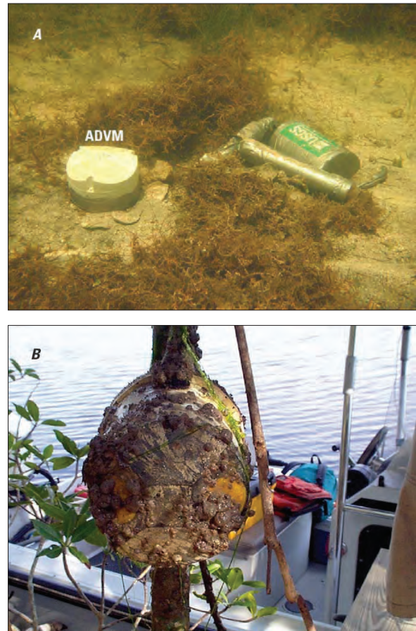
Figure 7. (A) Absence of biological fouling on an uplooker ADVm that has been treated with antifouling paint and (B) presence of biological fouling on an untreated sidelooker ADVm. (Top photograph by Victor Levesque, USGS; bottom photograph by Lars Soderqvist, USGS.)
