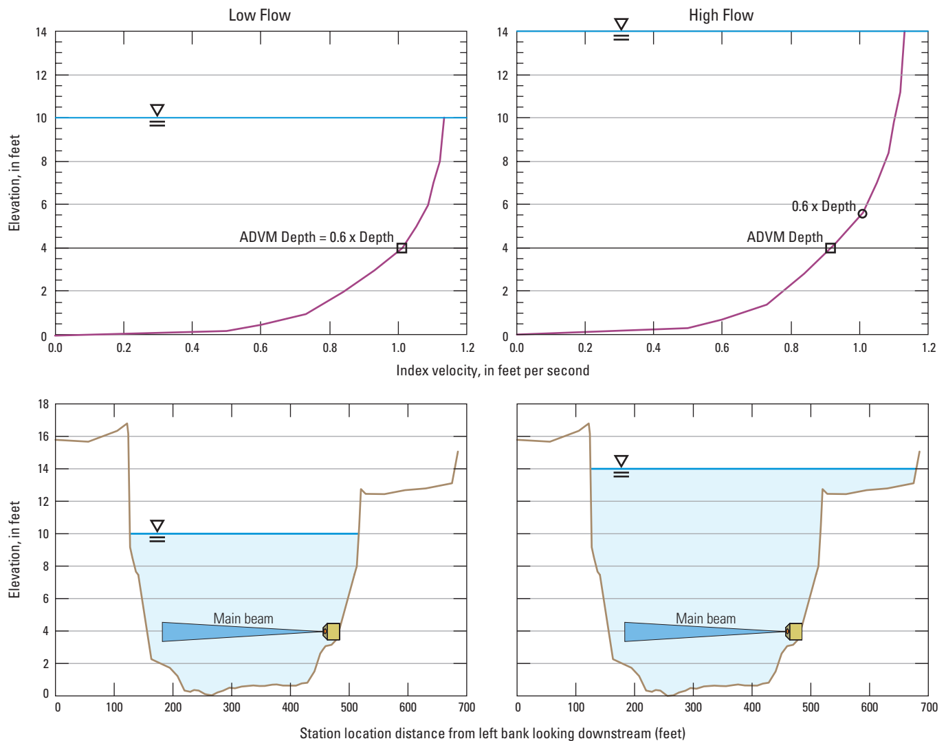
Figure 25. A water column velocity profile and possible change in the location of the ADVM measurement volume with changing stage.
