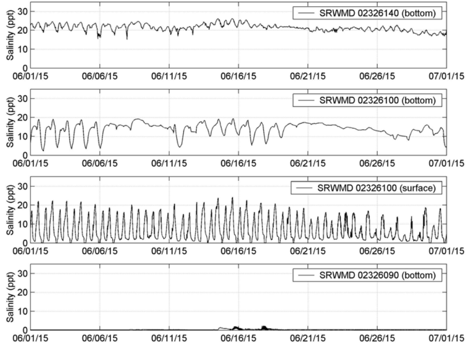
Figure 4-2e. Measured Salinity at Station SRWMD 02326140, 02326100, 02326090 (June 2015)
