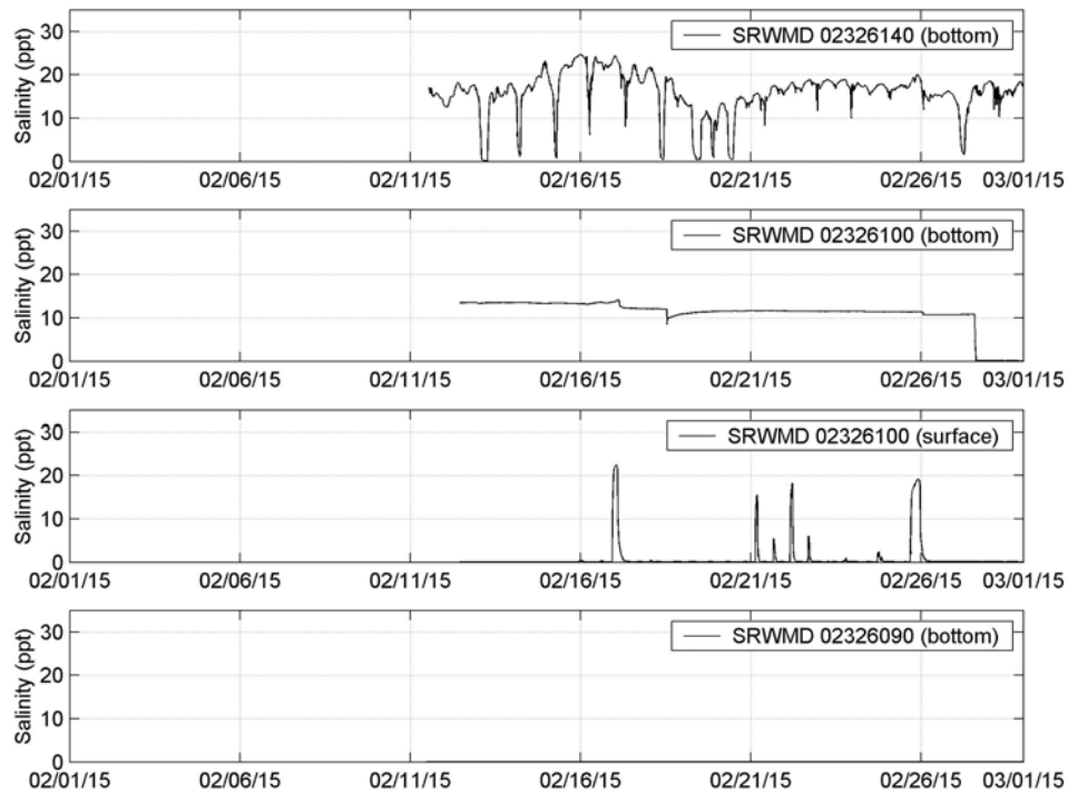
Figure 4-2a. Measured Salinity at Station SRWMD 02326140, 02326100, 02326090 (February 2015)
