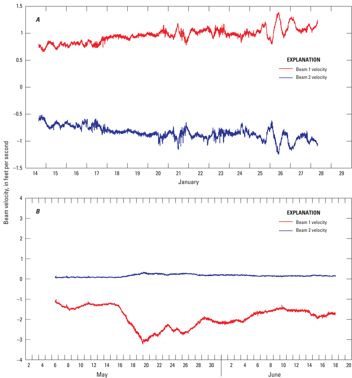
Figure 6. Beam velocity data from (A) a properly aligned sidelooker ADVM and (B) an improperly aligned sidelooker ADVM.
