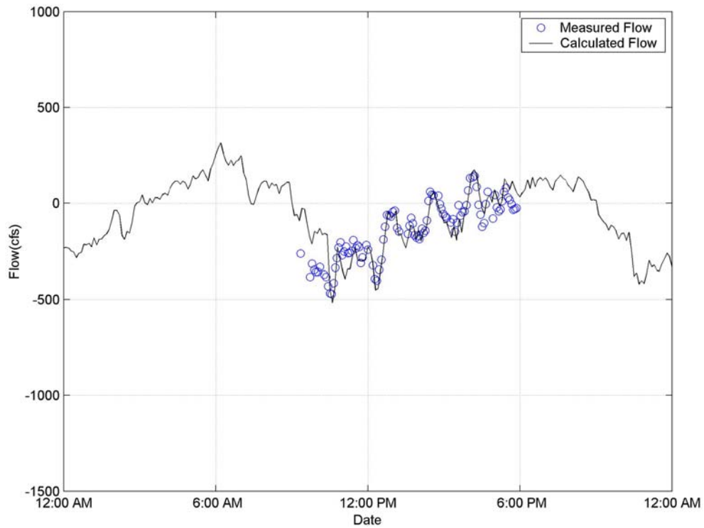
Figure 3-2. Measured and Calculated Flow on May 11, 2015
