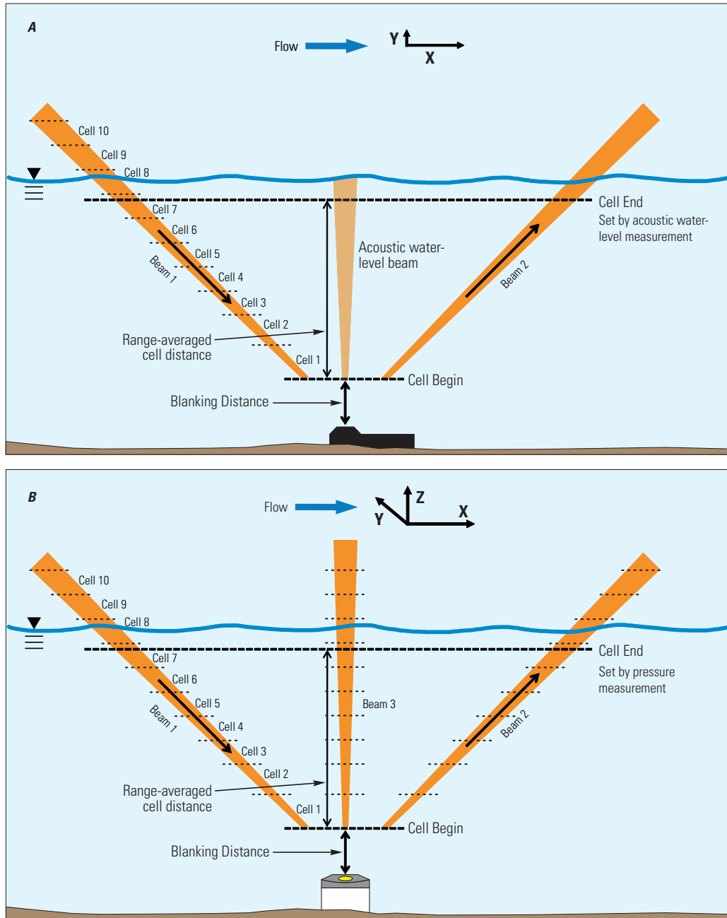
Figure 14. Generalized measurement volume for a (A) two-beam and (B) three-beam uplooker ADV.
