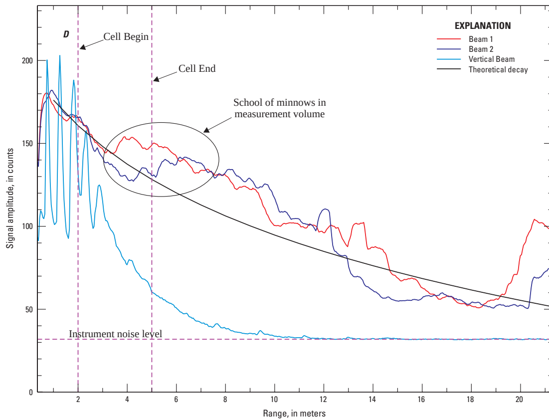
Figure 16—Continued. Results of beam checks showing data collected with (A) objects in the measurement volume, (B) side-lobe interference, (C) failed transducers, and (D) a school of minnows in the measurement volume.
