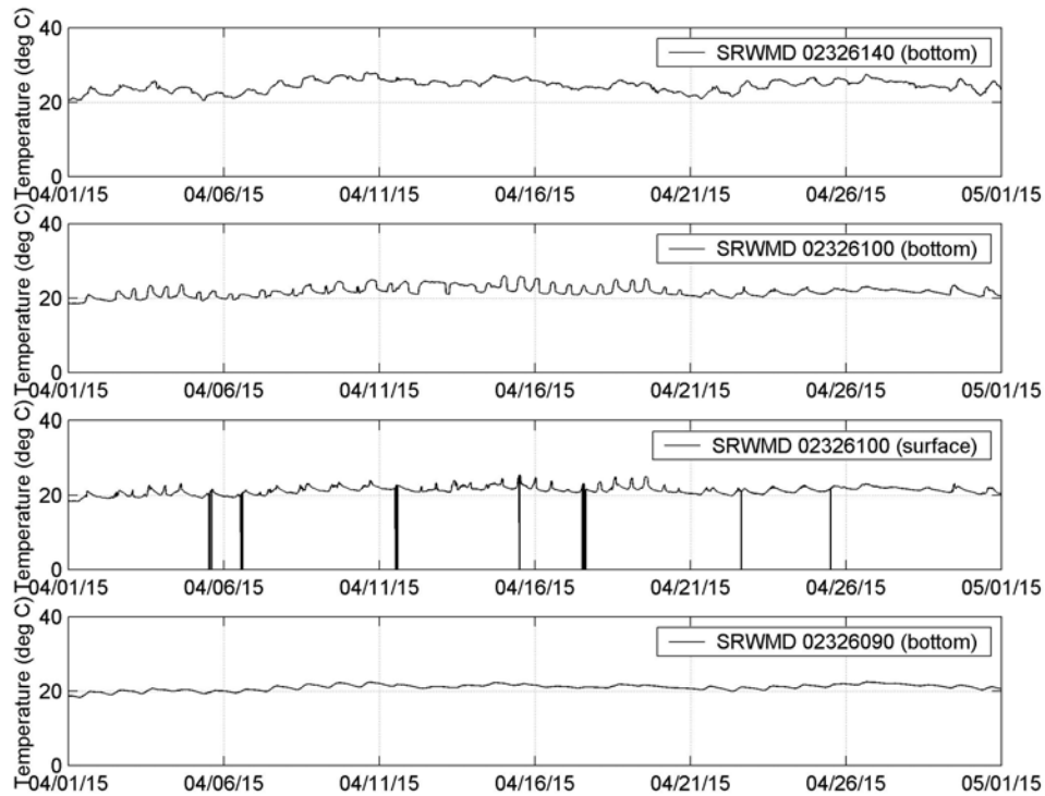
Figure 4-3c. Measured Temperature at Station SRWMD 02326140, 02326100, 02326090 (April 2015)
