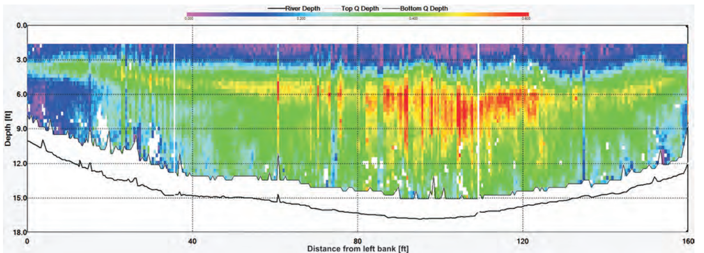
Figure 3. Channel cross section looking downstream with a uniform channel shape and an unusual velocity distribution from an ADCP reconnaissance measurement.
