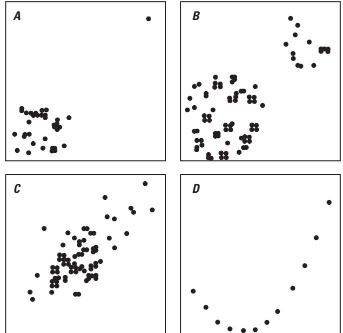
Figure 26. Scatter plots with the same coefficient of determination ( R^2 ) value (modified from Chambers and others, 1983).
