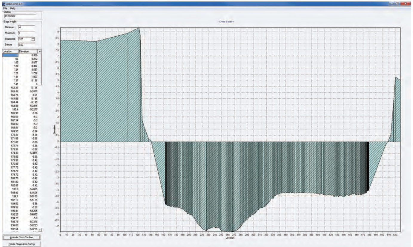
Figure 20. Cross-section data shown in U.S. Geological Survey AreaComp software.
