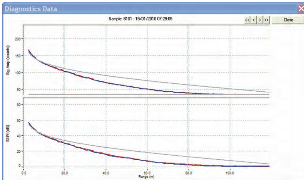
Figure 13. Change in cell end from automatic beam check diagnostic in January 2010. (Data from same site used in figure 11.)
