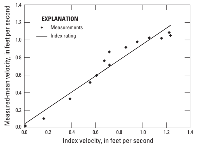
Figure 35. Plot showing curvature in the relation between index velocity and measured-mean velocity.
