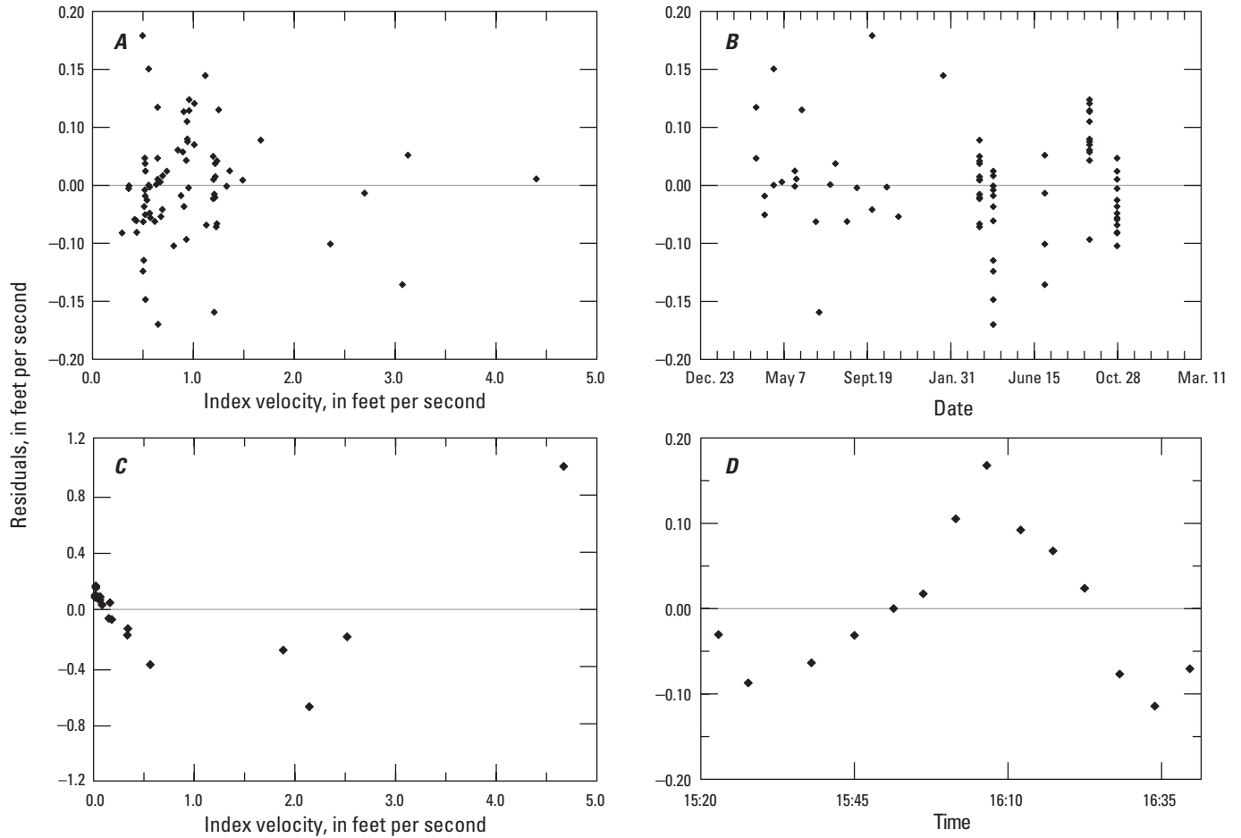
Figure 27. Residuals with no trend in (A) index velocity and (B) date; and residuals with a trend in (C) index velocity, and (D) time.
