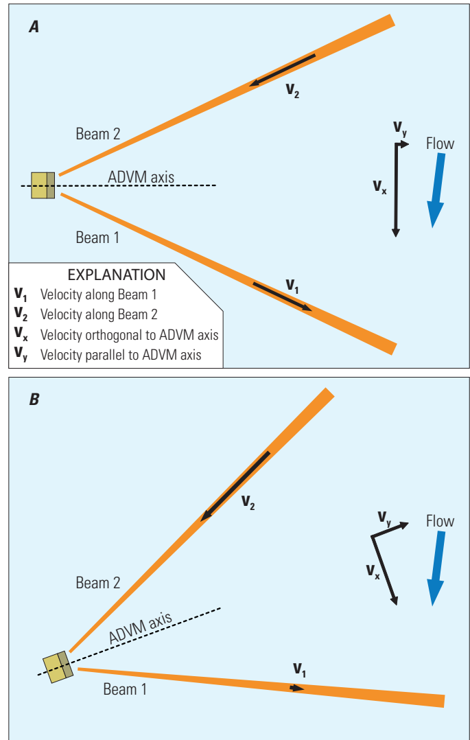
Figure 5. Plan view schematic of a sidelooker ADV (A) properly aligned to measure downstream and cross-stream velocity and (B) improperly aligned to measure downstream and cross-stream velocity. [ V_1 , Velocity along beam 1; V_2 , Velocity along beam 2; V_x , Velocity orthogonal to ADVM axis; V_y , Velocity parallel to ADVM axis].
