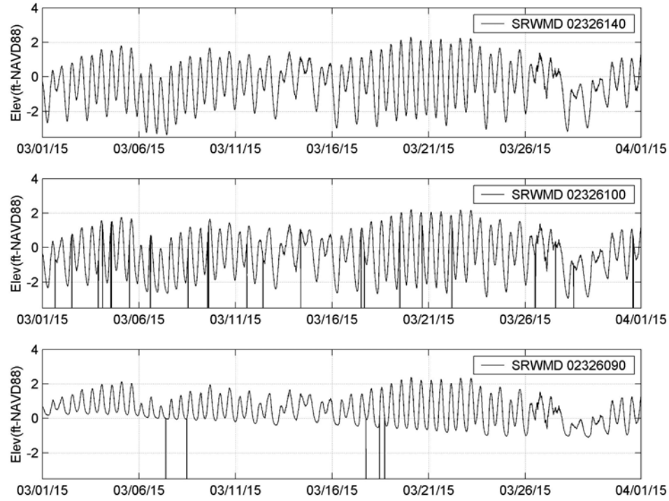
Figure 4-1b. Measured Water Level at Station 02326140, 02326100, 02326090 (March 2015)
