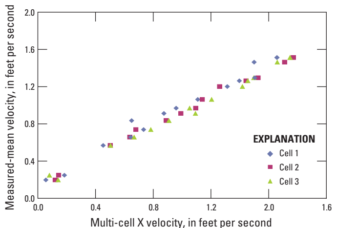
Figure 24. Multi-cell index velocity data with measured-mean velocity.
