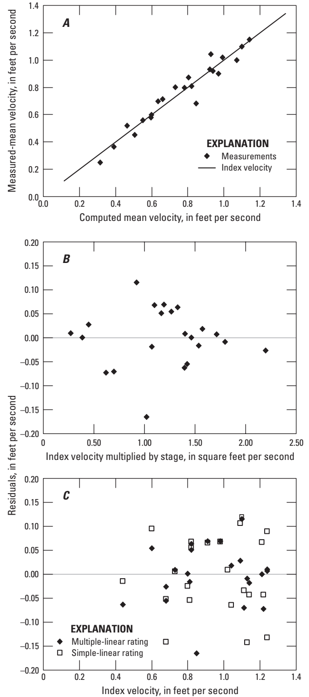
Figure 40. Plots of (A) measured-mean velocity with computed mean velocity and residuals with (B) stage multiplied by index velocity and (C) index velocity for multiple-linear regression using index velocity and stage multiplied by index velocity as independent variables.
