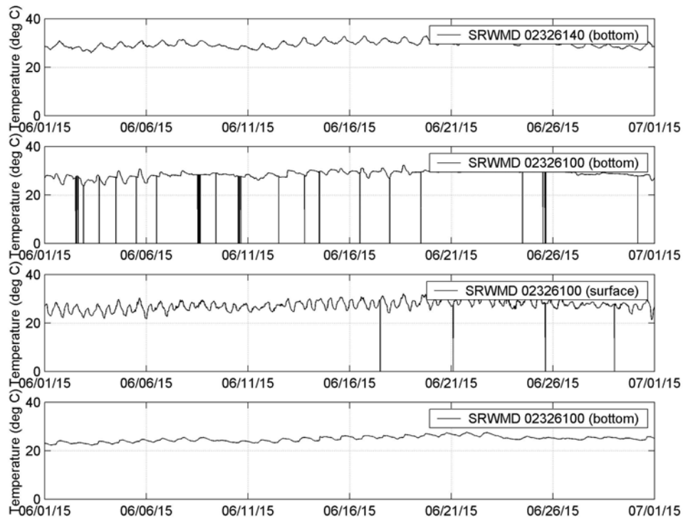
Figure 4-3e. Measured Temperature at Station SRWMD 02326140, 02326100, 02326090 (June 2015)
