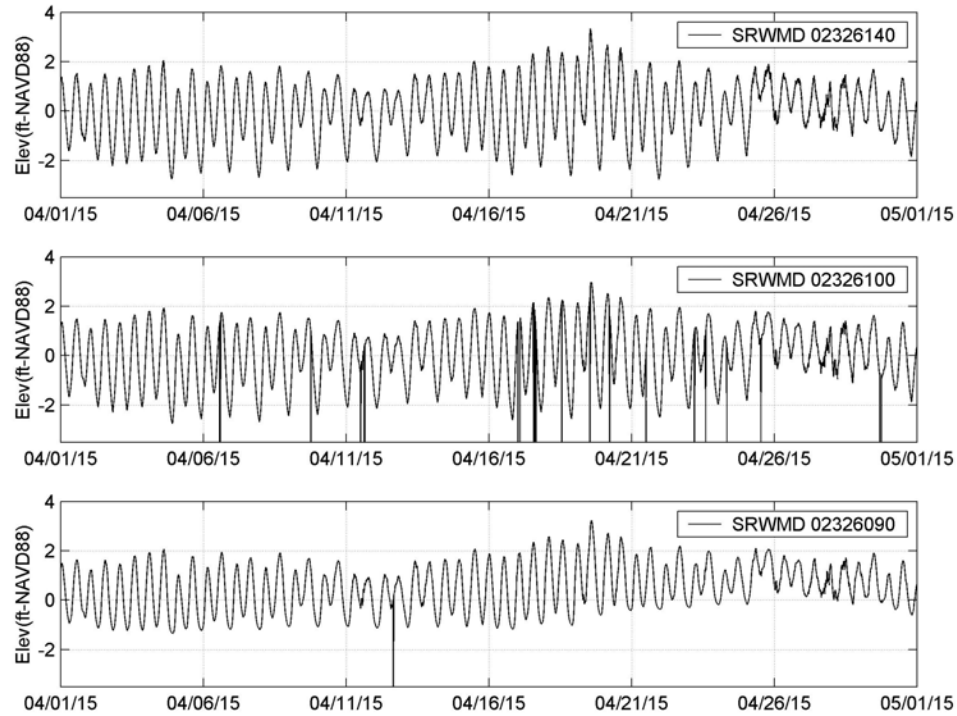
Figure 4-1c. Measured Water Level at Station 02326140, 02326100, 02326090 (April 2015)
