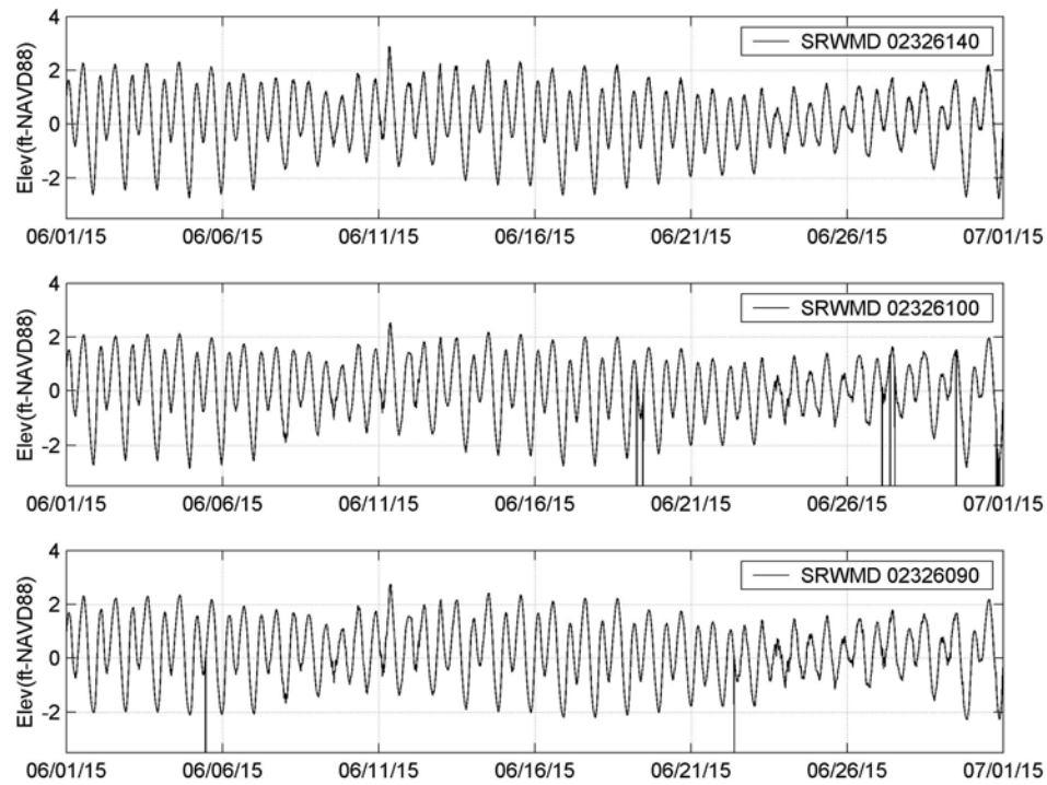
Figure 4-1e. Measured Water Level at Station 02326140, 02326100, 02326090 (June 2015)
