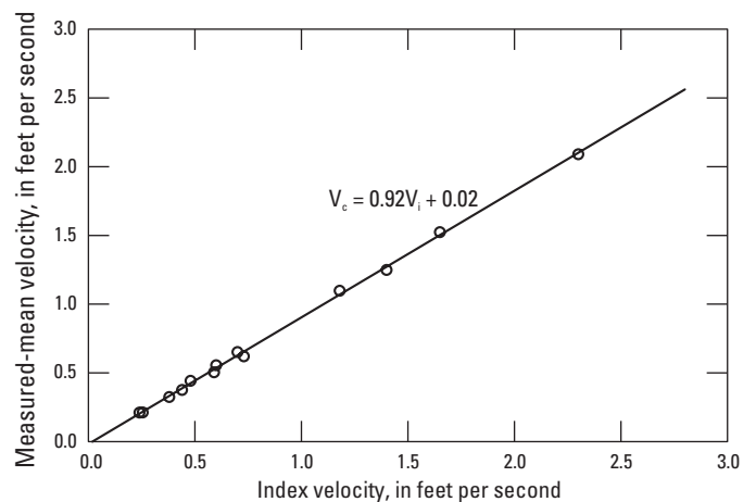
Figure 22. Example of an index rating.
