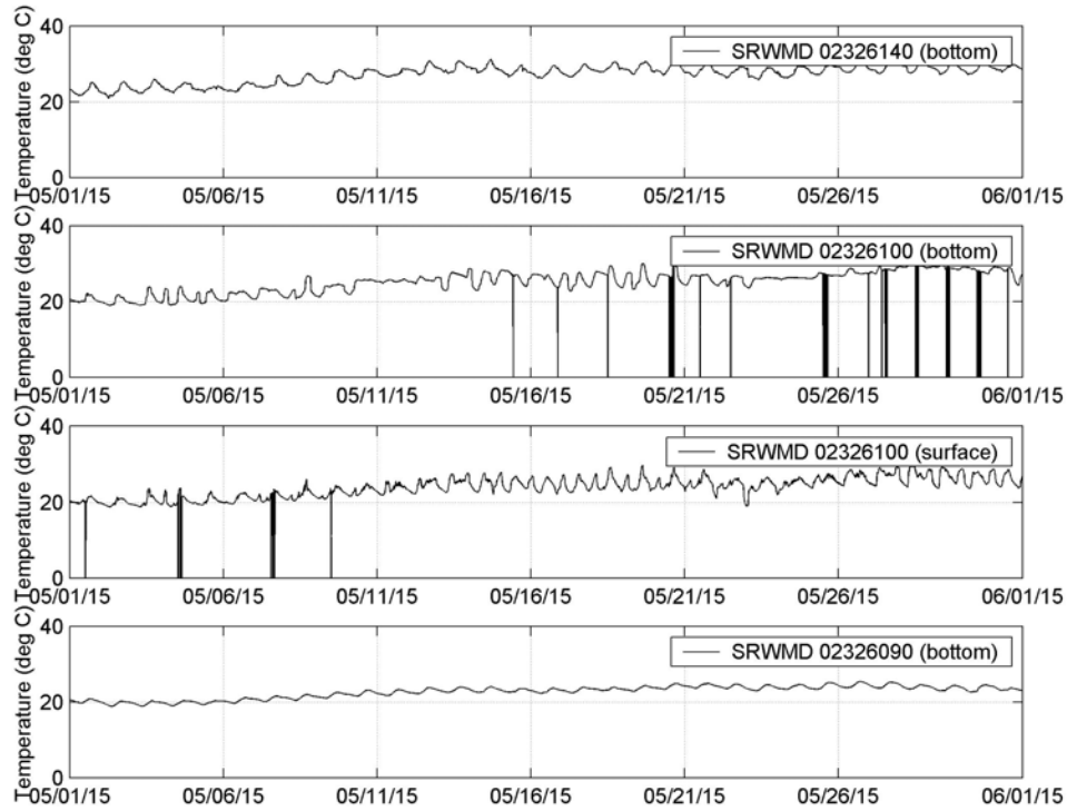
Figure 4-3d. Measured Temperature at Station SRWMD 02326140, 02326100, 02326090 (May 2015)
