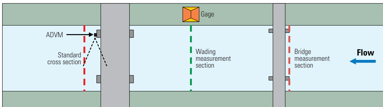
Figure 17. Schematic showing location of standard cross section at an index velocity station.
