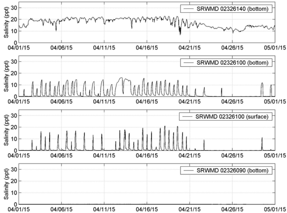
Figure 4-2c. Measured Salinity at Station SRWMD 02326140, 02326100, 02326090 (April 2015)
