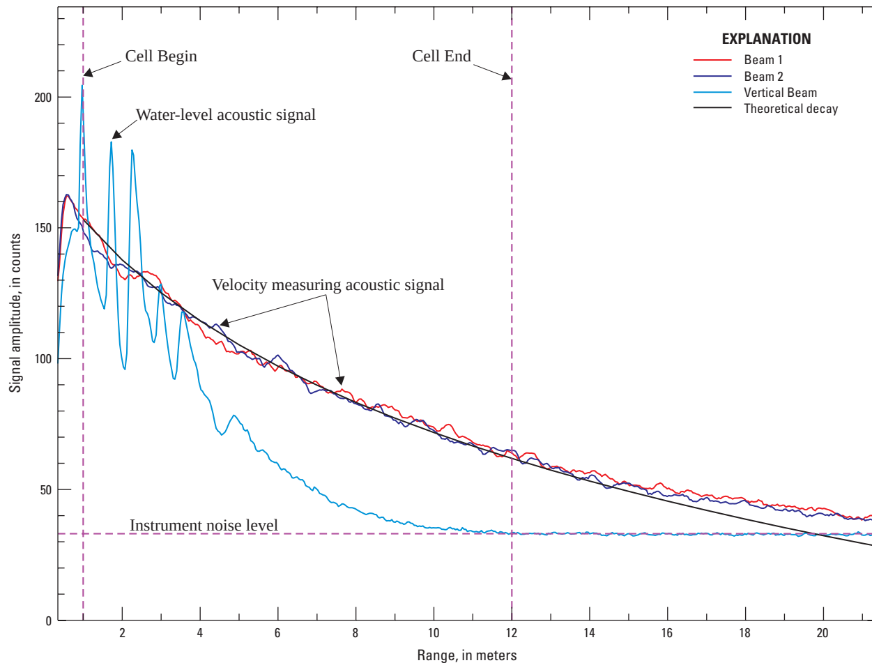
Figure 9. An example of a signal amplitude (beam) check for a sidelooker ADVM with a water-level acoustic beam.
