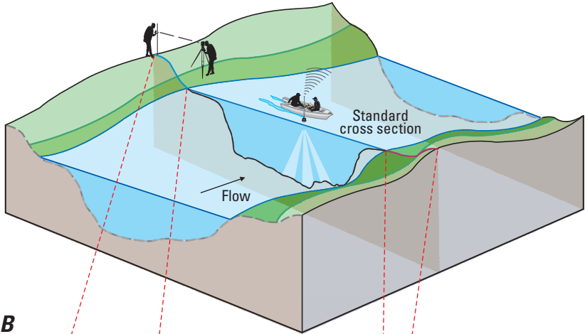
Figure 19. Combined stage-area survey created from (A) standard surveying techniques on shore (table 4) and a vessel-mounted acoustic Doppler current profiler (ADCP) used to capture channel bathymetry along measured cross sections (table 5) and (B) cross section derived from combined shore survey with ADCP channel bathymetry (diagram modified from Ruhl and Simpson, 2005).
