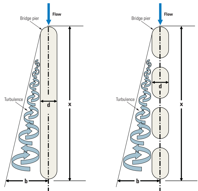
Figure 10. Theoretical bridge pier-wake turbulence dimensions.
