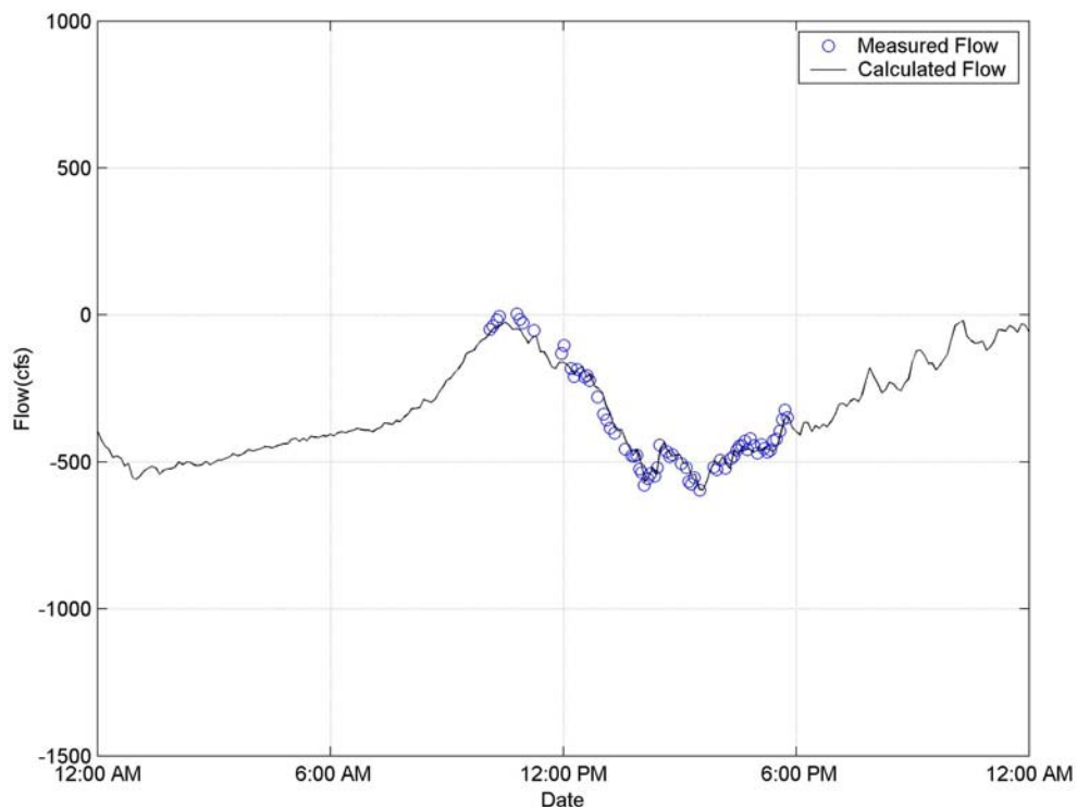
Figure 3-1. Measured and Calculated Flow on March 17, 2015
