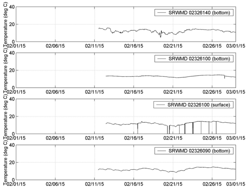
Figure 4-3a. Measured Temperature at Station SRWMD 02326140, 02326100, 02326090 (February 2015)
