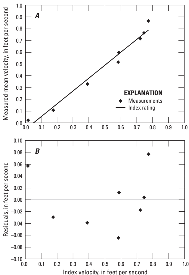
Figure 32. Plots of (A) measured-mean velocity and index velocity, and (B) regression residuals with index velocity for lower range of compound-linear rating example.
