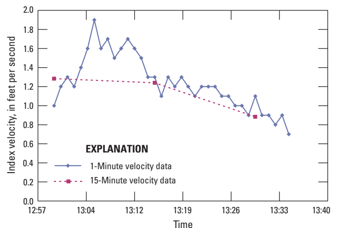
Figure 15. Effect of using different measurement intervals and averaging periods.
