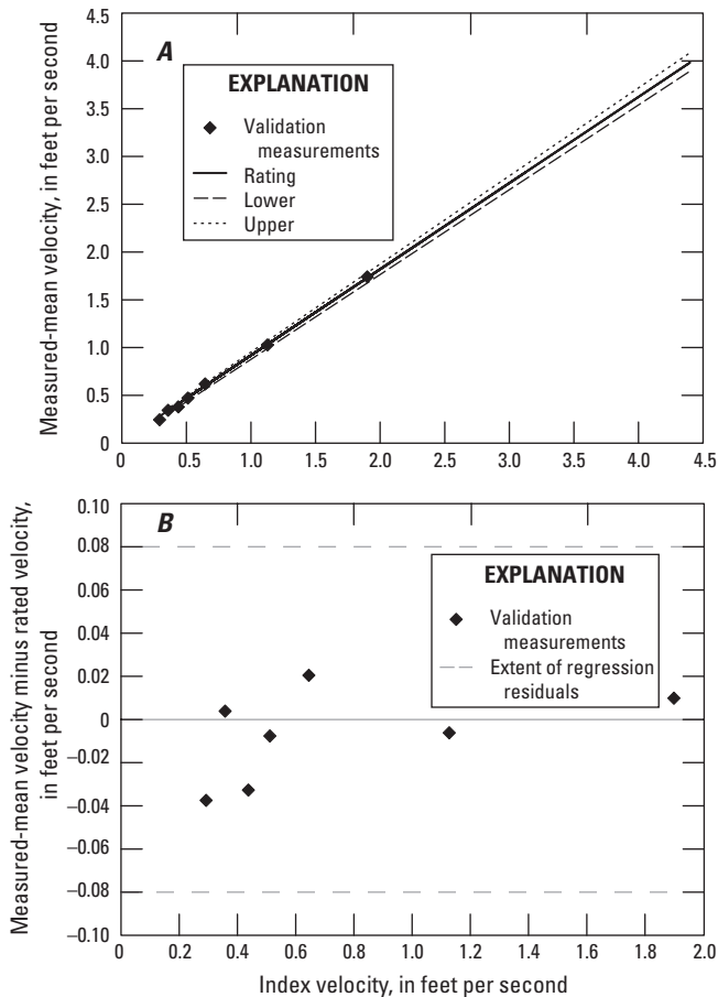
Figure 41. Scatter plot and residuals plot for validation measurements.
