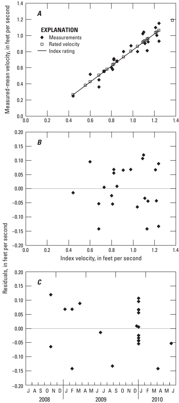
Figure 39. Plots of (A) measured-mean velocity and predicted mean velocity and regression residuals from simple-linear regression with (B) index velocity and (C) measurement date for multiple-linear regression example.
