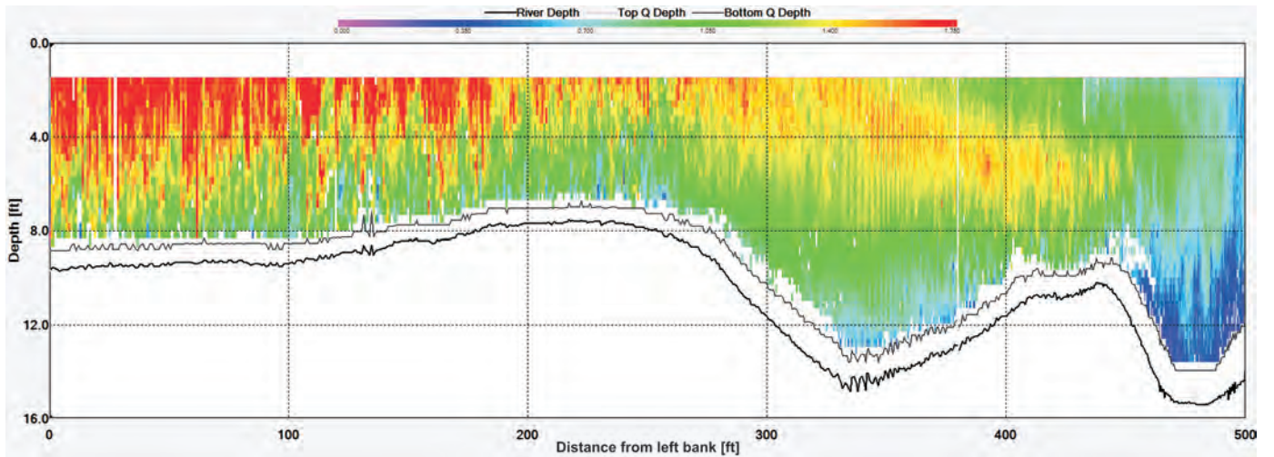
Figure 1. Channel cross section looking downstream with a non-uniform channel shape and non-uniform velocity distribution from an ADCP reconnaissance measurement.
