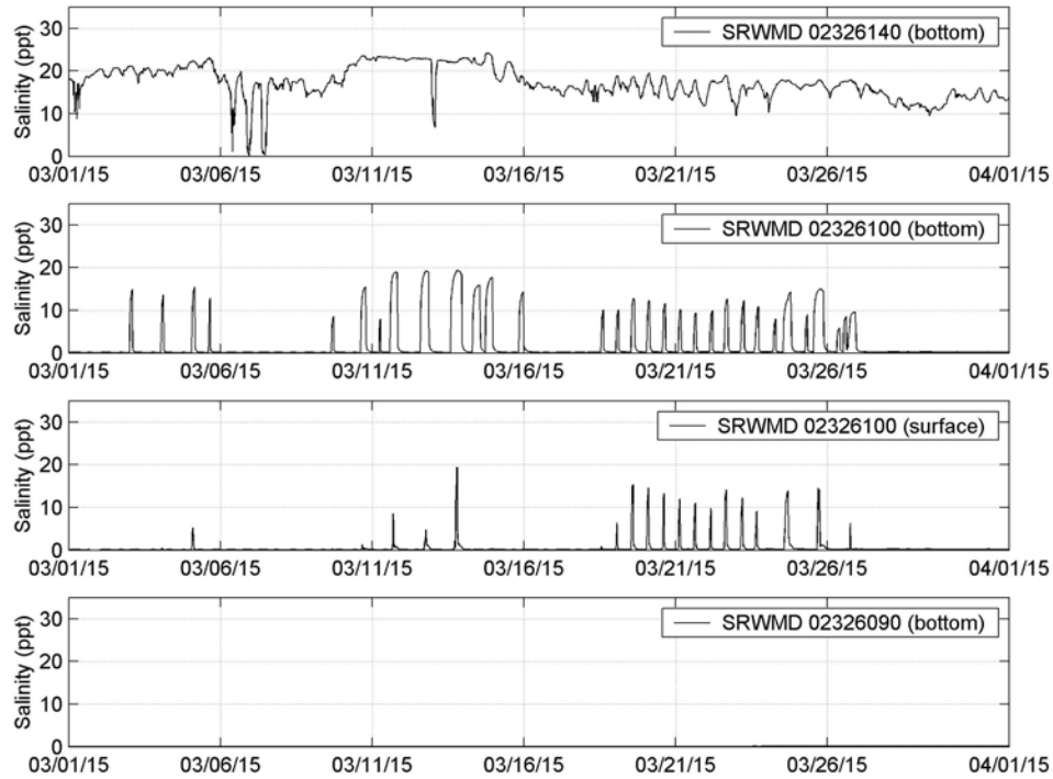
Figure 4-2b. Measured Salinity at Station SRWMD 02326140, 02326100, 02326090 (March 2015)
