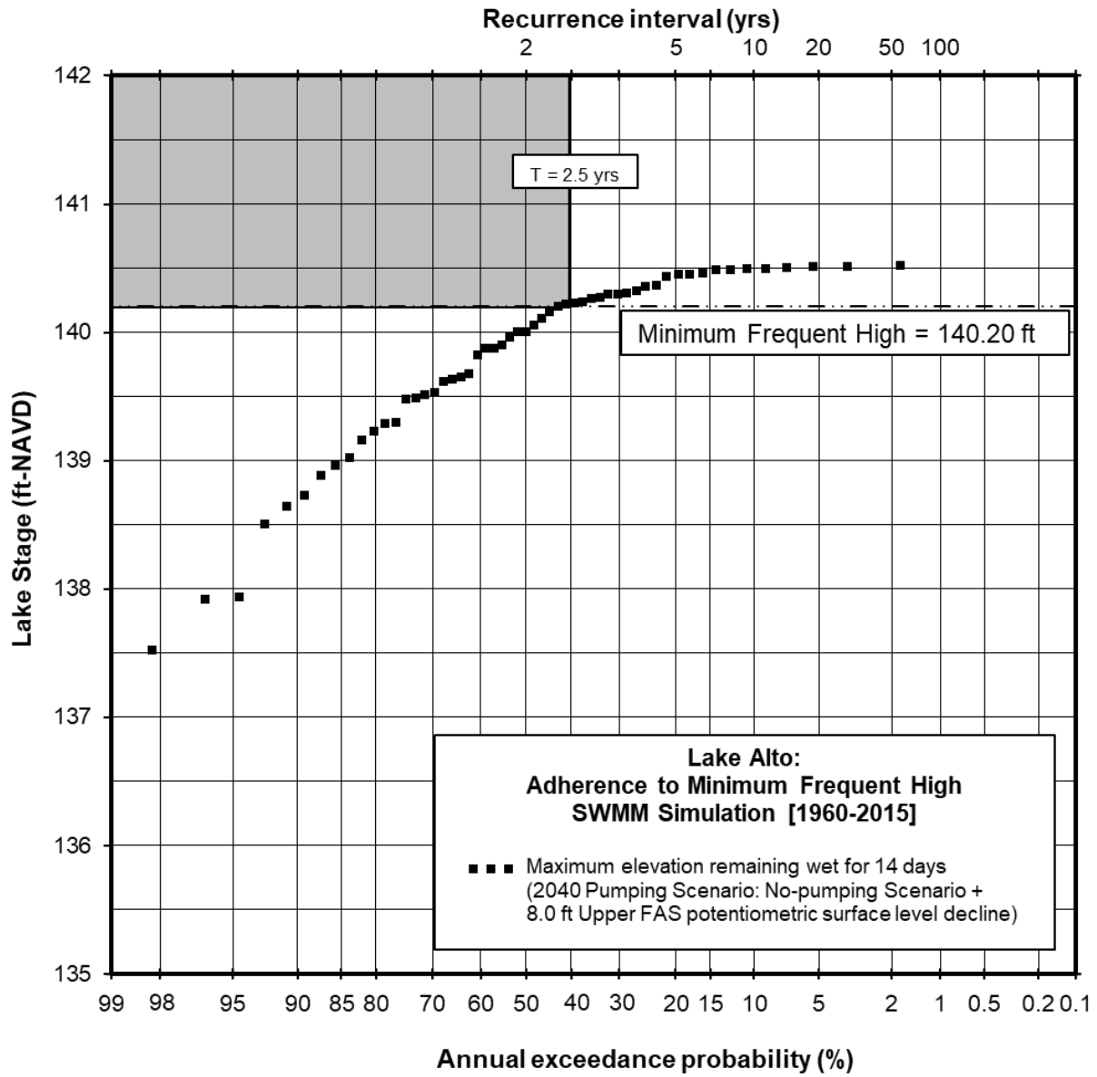
Figure 7. Lake Alto Minimum Frequent High Level and Model-Simulated Lake Stage Data Set (1960-2015) – 2040 Pumping Scenario.
