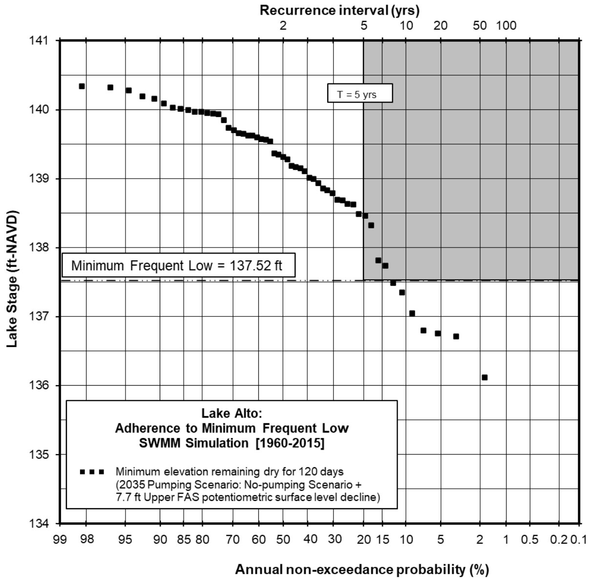
Figure 6. Lake Alto Minimum Frequent Low Level and Model-Simulated Lake Stage Data Set (1960-2015) – 2035 Pumping Scenario.
