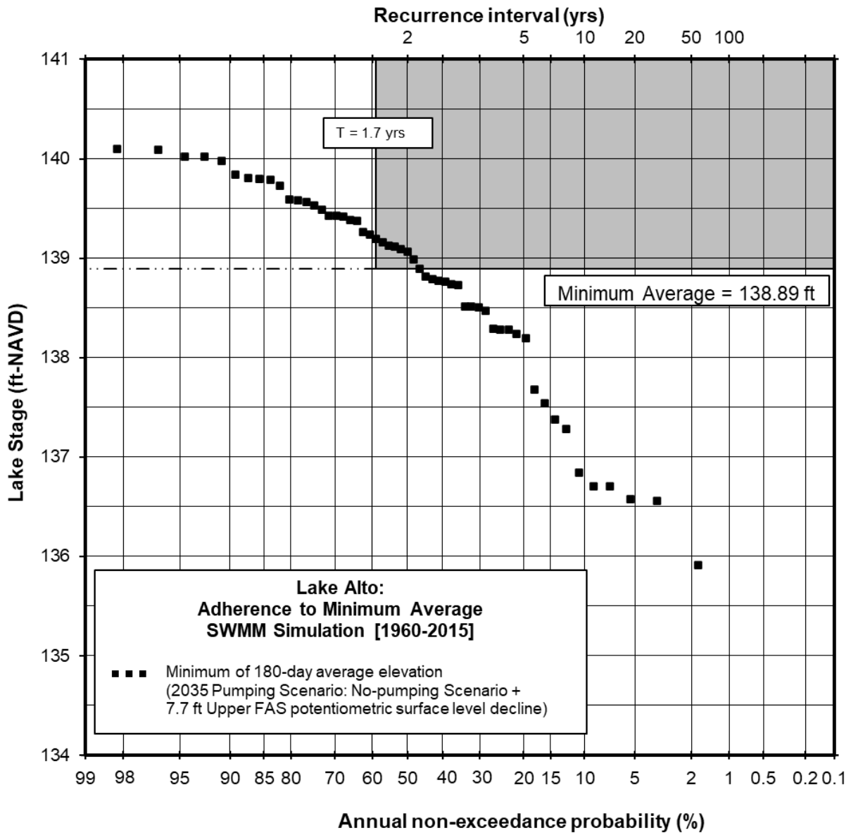
Figure 5. Lake Alto Minimum Average Level and Model-Simulated Lake Stage Data Set (1960-2015) – 2035 Pumping Scenario.
