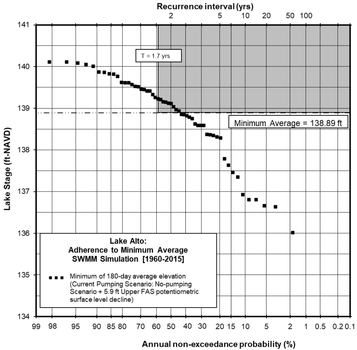
Figure 2. Lake Alto Minimum Average Level and Model-Simulated Lake Stage Data Set (1960-2015) – Current Pumping Scenario.
