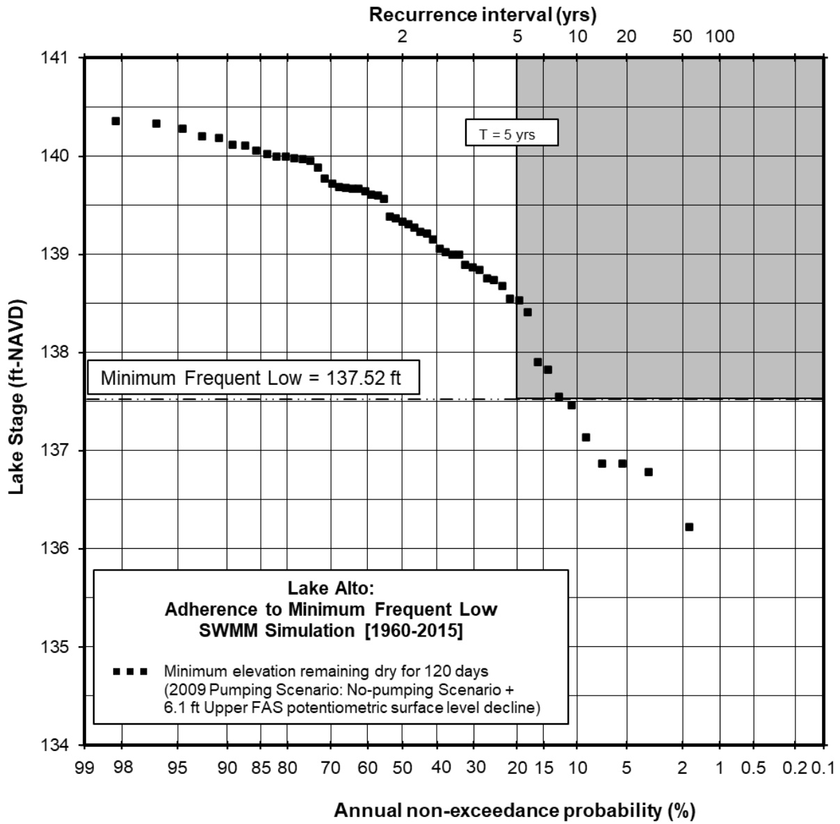
Figure A-3. Lake Alto Minimum Frequent Low Level and Model-Simulated Lake Stage Data Set (1960-2015) – 2009 Pumping Scenario.
