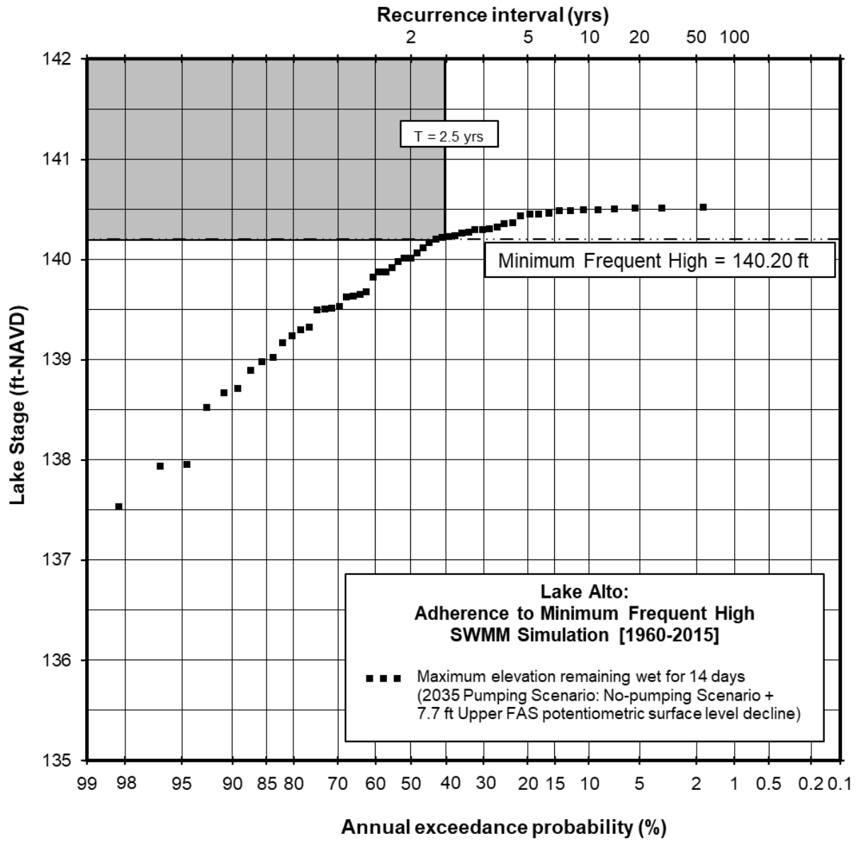
Figure 4. Lake Alto Minimum Frequent High Level and Model-Simulated Lake Stage Data Set (1960-2015) – 2035 Pumping Scenario.
