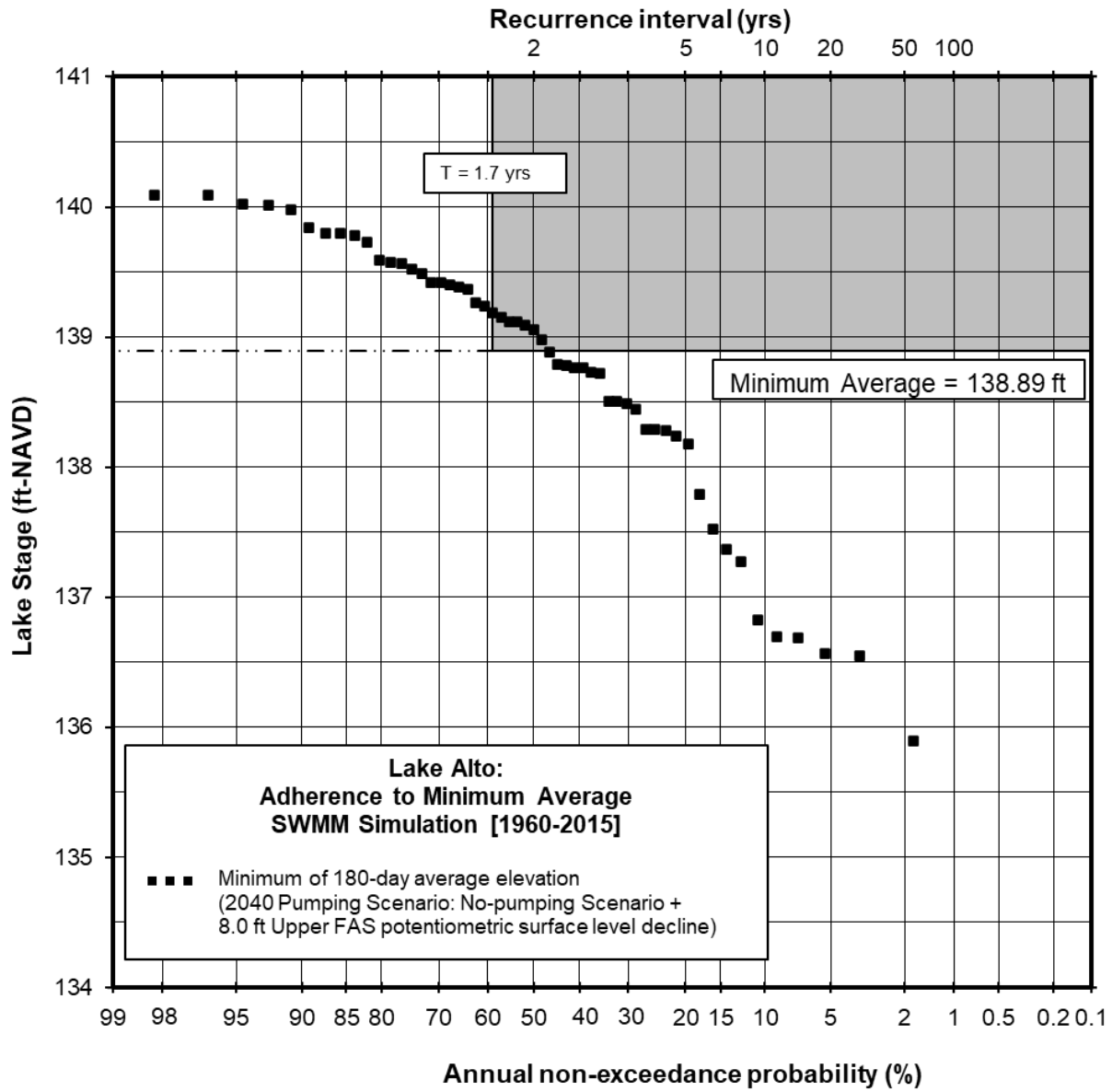
Figure 8. Lake Alto Minimum Average Level and Model-Simulated Lake Stage Data Set (1960-2015) – 2040 Pumping Scenario.
