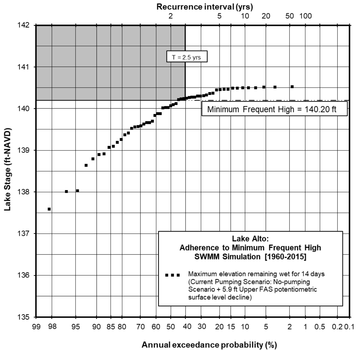
Figure 1. Lake Alto Minimum Frequent High Level and Model-Simulated Lake Stage Data Set (1960-2015) – Current Pumping Scenario.
