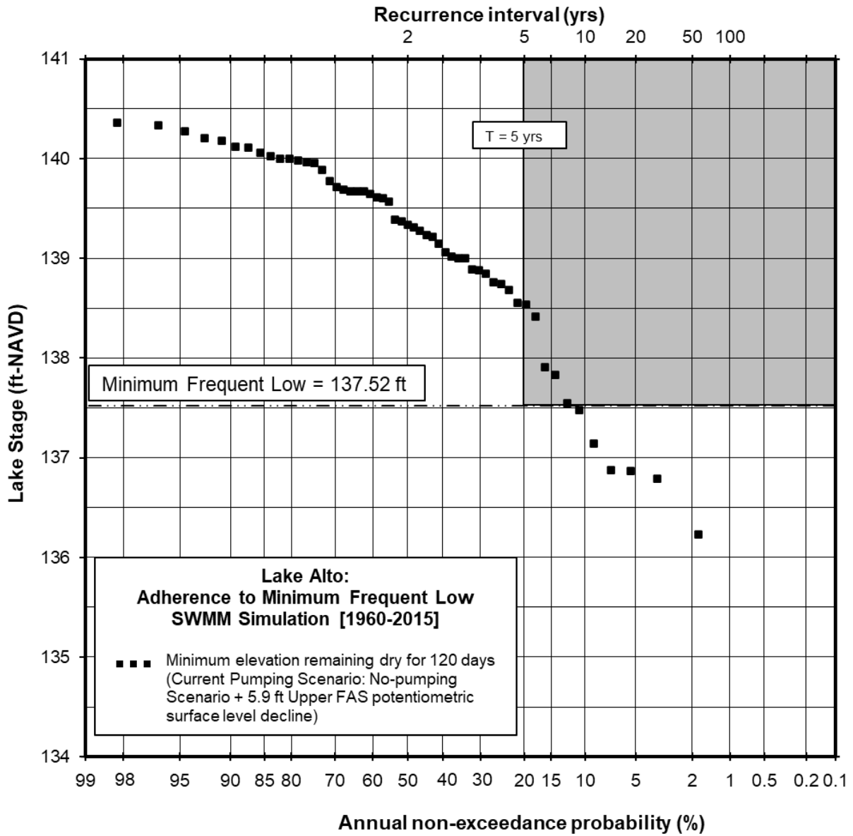
Figure 3. Lake Alto Minimum Frequent Low Level and Model-Simulated Lake Stage Data Set (1960-2015) – Current Pumping Scenario.
