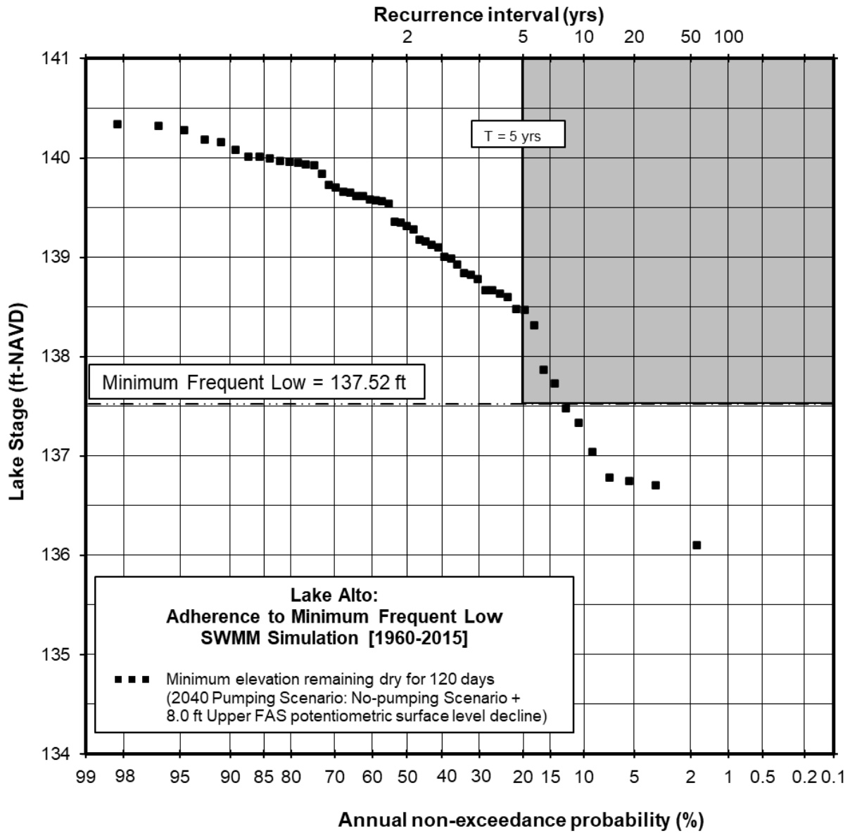
Figure 9. Lake Alto Minimum Frequent Low Level and Model-Simulated Lake Stage Data Set (1960-2015) – 2040 Pumping Scenario.
