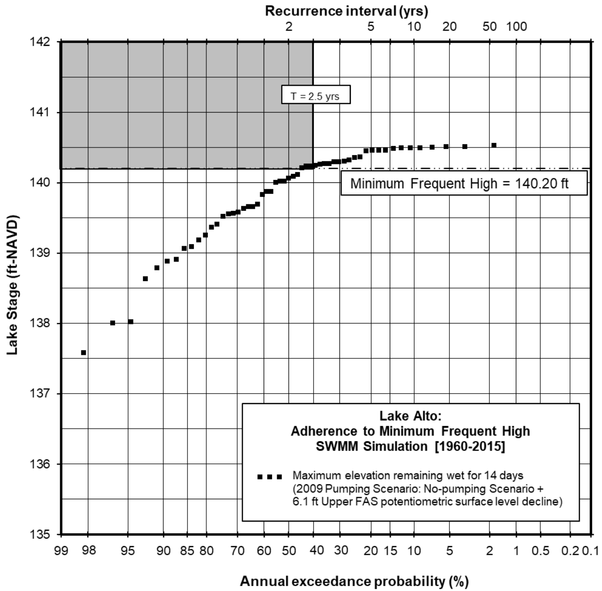
Figure A-1. Lake Alto Minimum Frequent High Level and Model-Simulated Lake Stage Data Set (1960-2015) – 2009 Pumping Scenario.
