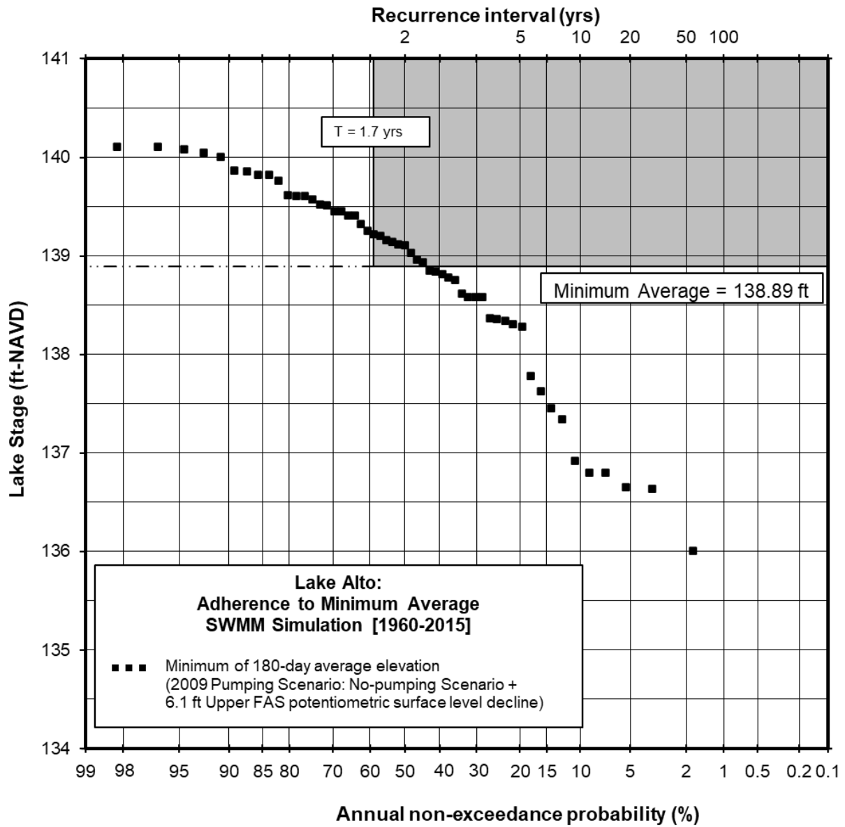
Figure A-2. Lake Alto Minimum Average Level and Model-Simulated Lake Stage Data Set (1960-2015) – 2009 Pumping Scenario.
