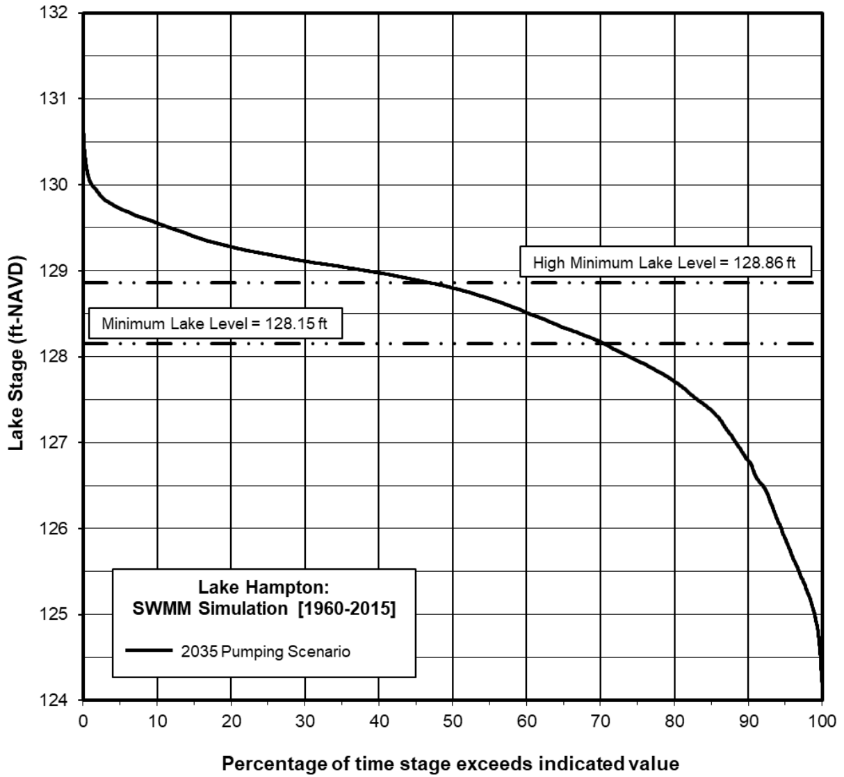
Figure 2. Stage Duration Curve of Model-Simulated Lake Stage Data Set (1960-2015) for 2035 Pumping Scenario and Recommended Minimum levels for Lake Hampton.
