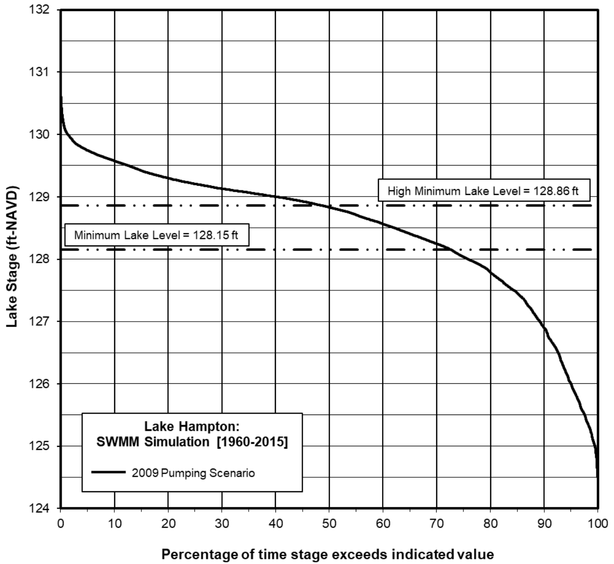
Figure A-1. Stage Duration Curve of Model-Simulated Lake Stage Data Set (1960-2015) for 2009 Pumping Scenario and Recommended Minimum levels for Lake Hampton.
