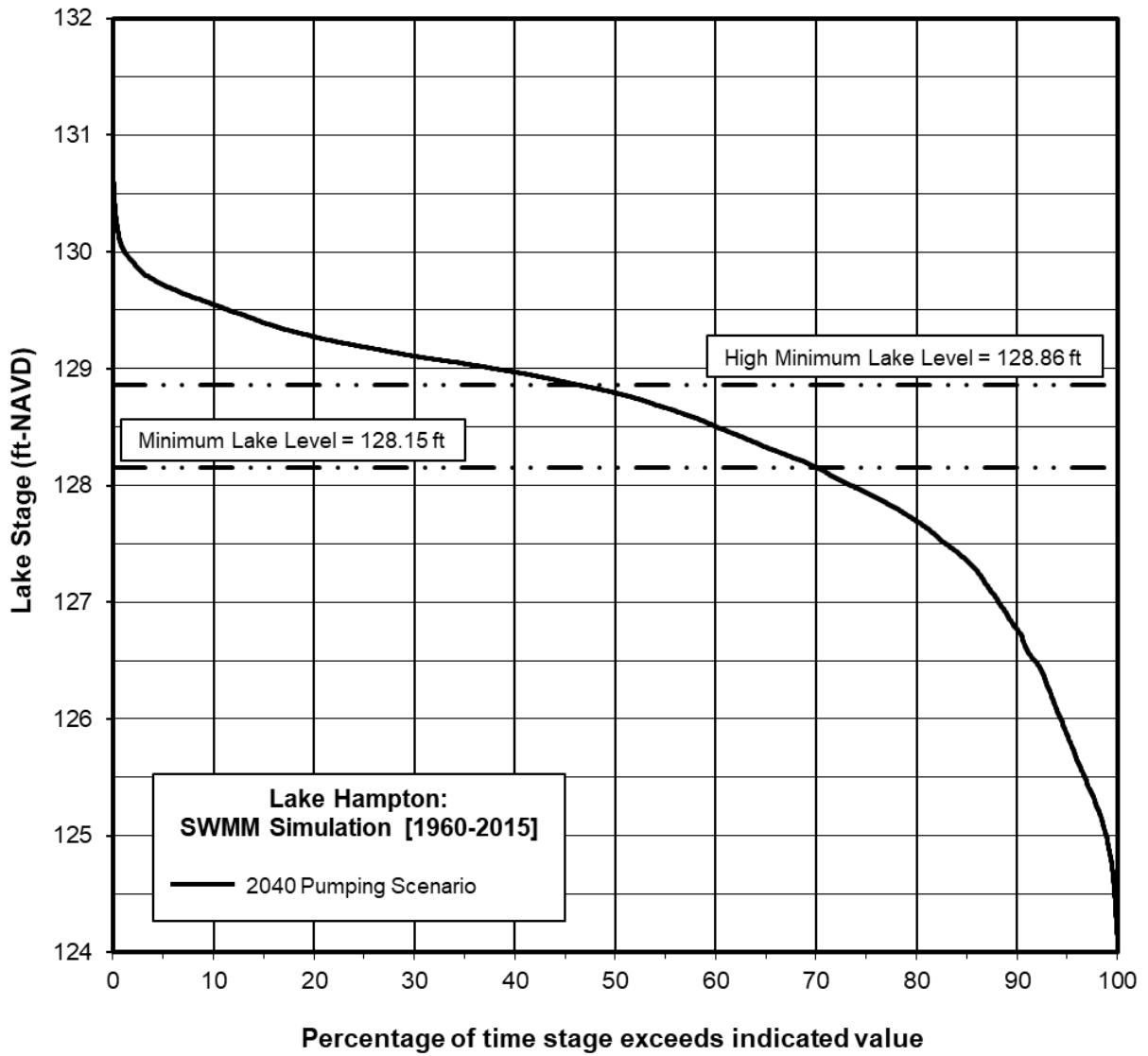
Figure 3. Stage Duration Curve of Model-Simulated Lake Stage Data Set (1960-2015) for 2040 Pumping Scenario and Recommended Minimum levels for Lake Hampton.
