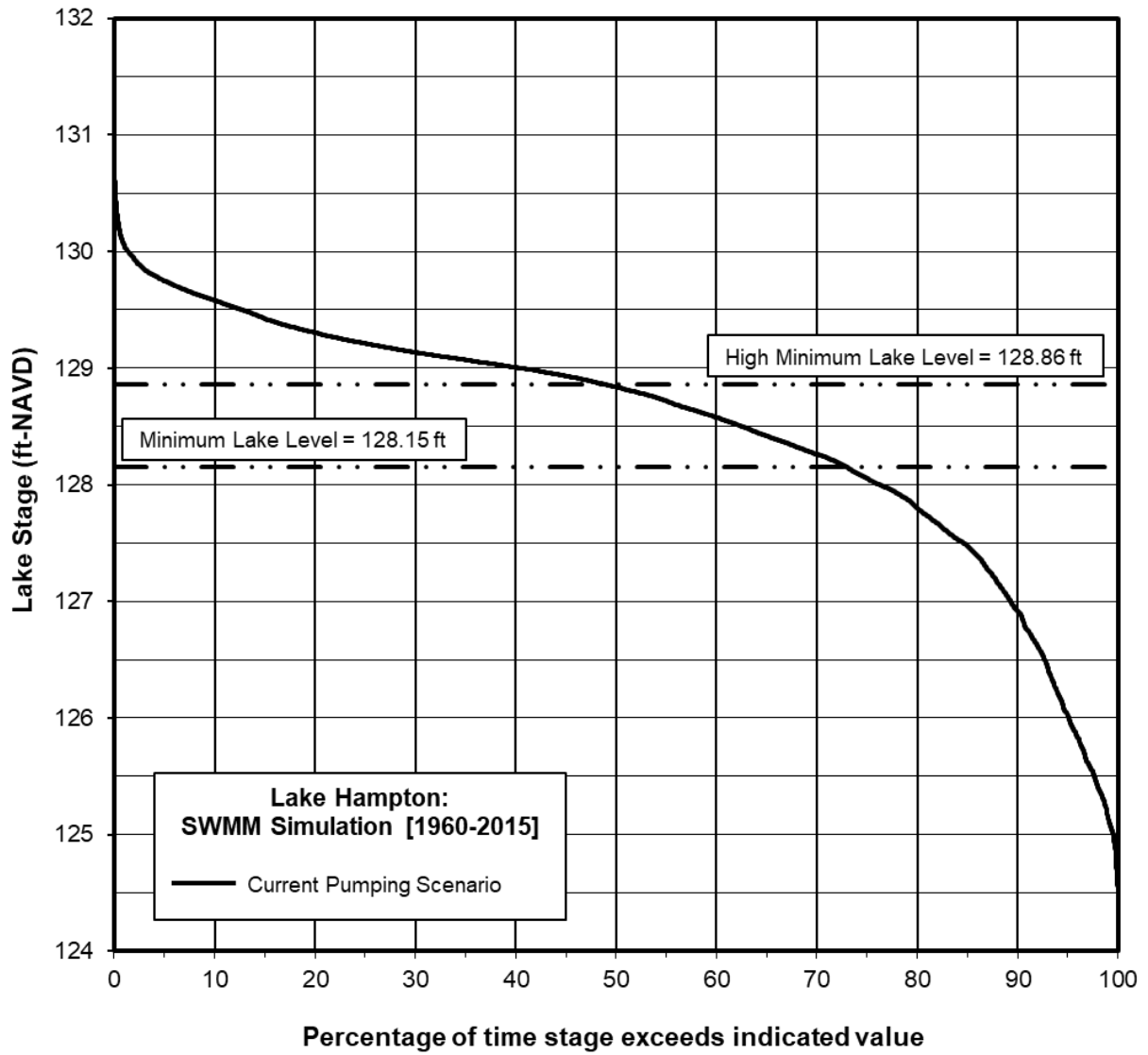
Figure 1. Stage Duration Curve of Model-Simulated Lake Stage Data Set (1960-2015) for Current Pumping Scenario and Recommended Minimum levels for Lake Hampton.
